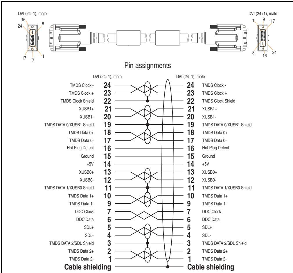
Figure 357: Pin assignments - SDL cable 5CASDL.0xxx-03
