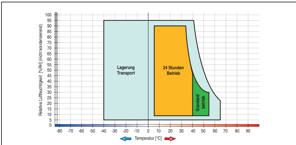
Figure 107: Temperature humidity diagram - RAID hard disk 5ACPCI.RAIS-01
