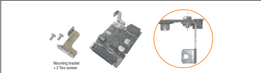
Figure 429: Install mounting bracket
