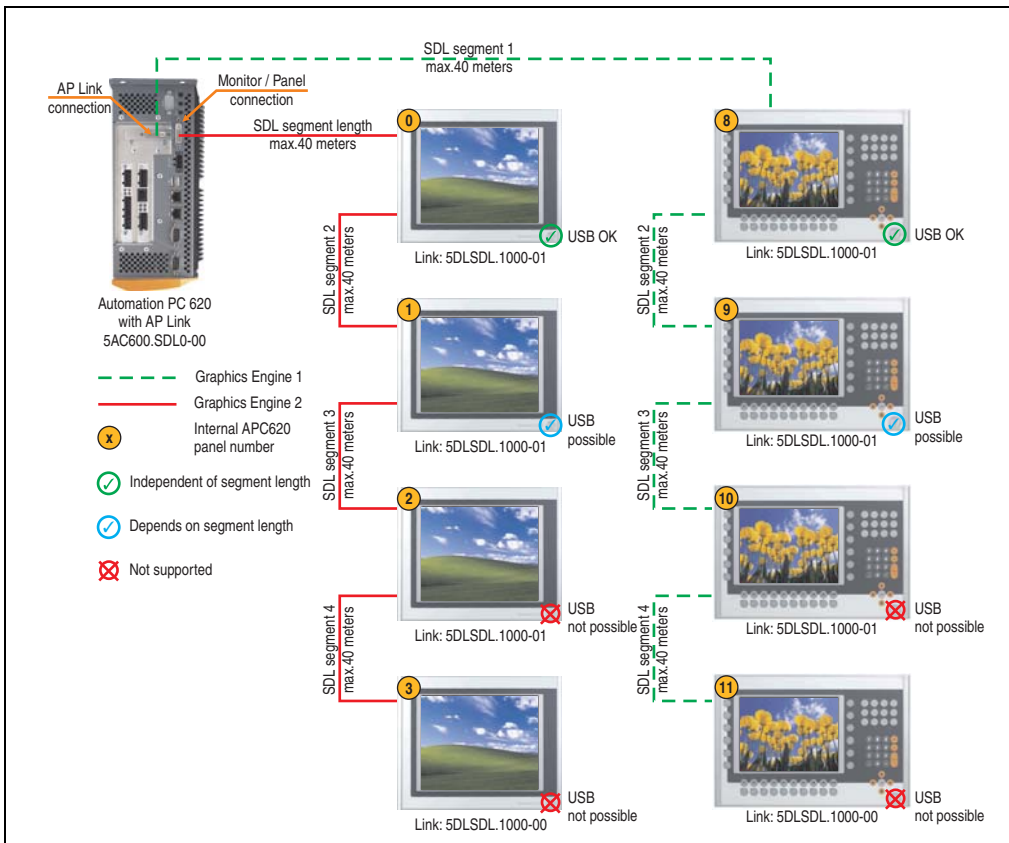
Figure 155: Configuration - Eight Automation Panel 900 units via SDL (onboard) and SDL (AP Link)
