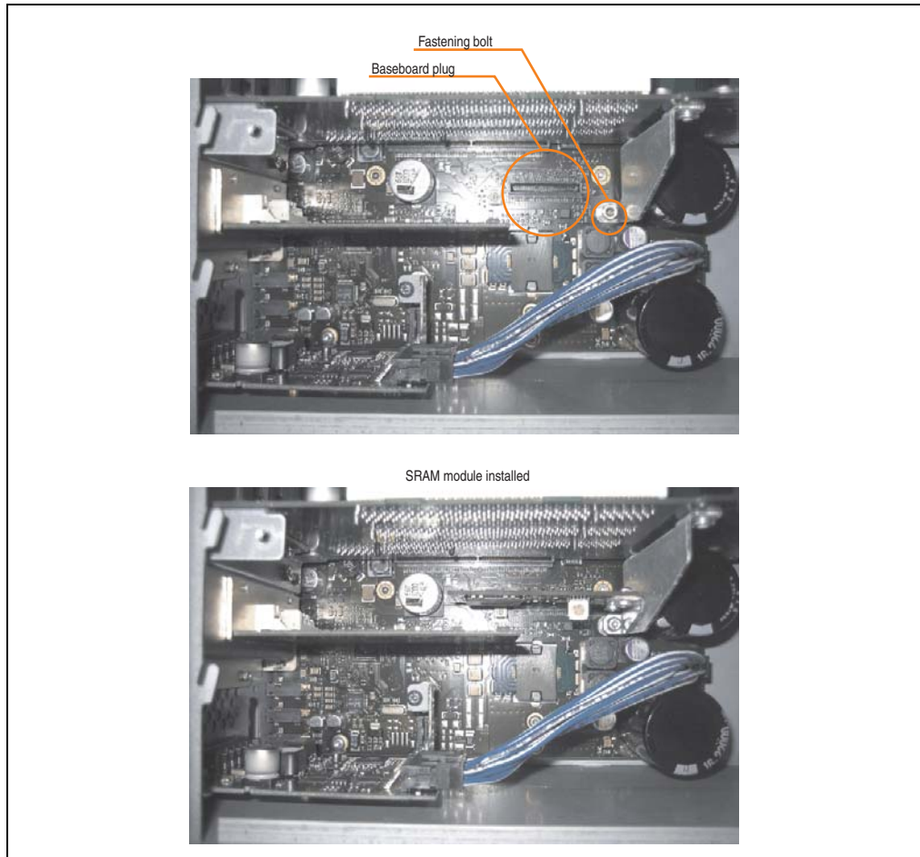
Figure 385: SRAM module installation
