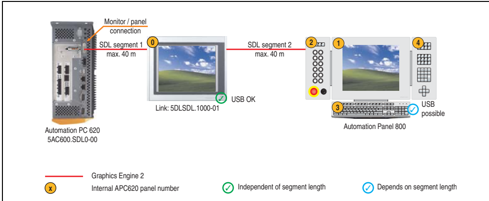
Figure 150: Configuration - One AP900 and an AP800 via SDL (onboard)
