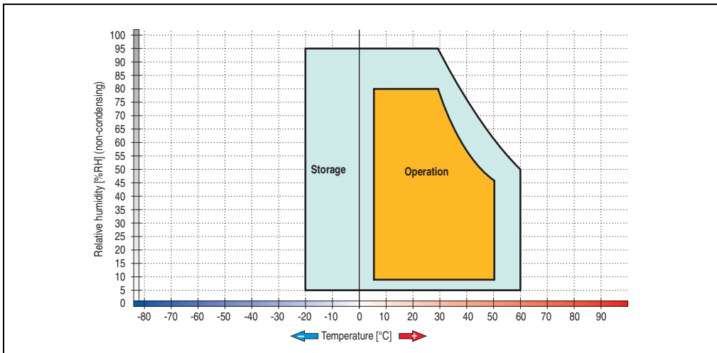
Figure 90: Temperature humidity diagram - Slide-in DVD-ROM/CD-RW 5AC600.DVDS-00
