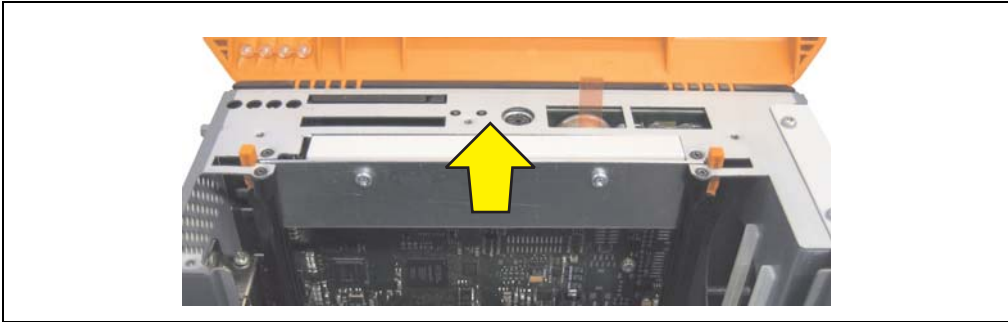
Figure 415: Removing the slide-in dummy module
