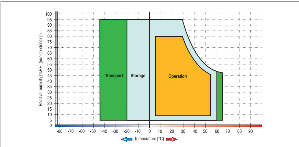
Figure 92: Temperature humidity diagram - Slide-in DVD-R/RW, DVD+R/RW 5AC600.DVRS-00
