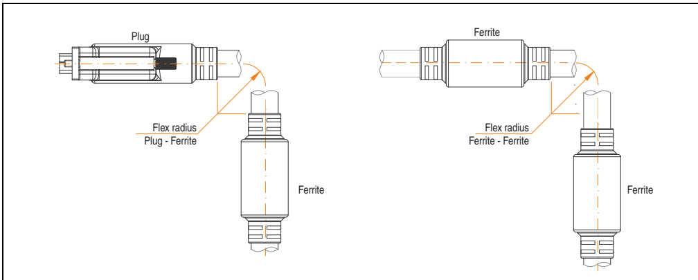
Figure 345: Flex radius specification
