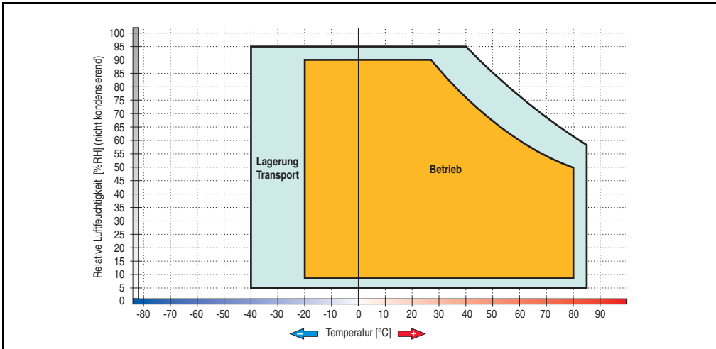
Figure 99: Temperature humidity diagram - Slide-in hard disk 5AC600.HDDS-01
