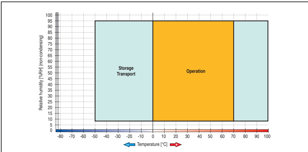
Figure 312: Temperature humidity diagram - CompactFlash cards 5CFCRD.xxxx-03
