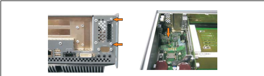
Figure 430: Install UPS module
