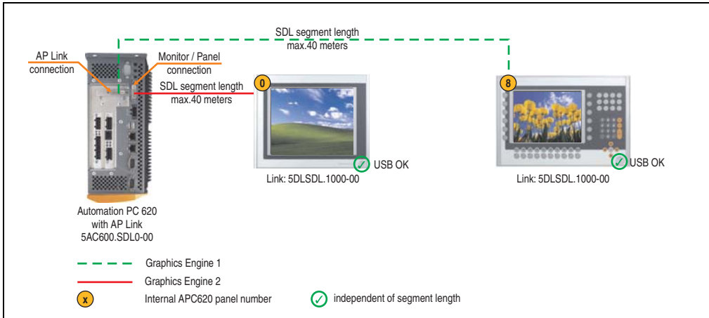
Figure 154: Configuration - Two Automation Panel 900 units via SDL (onboard) and SDL (AP Link)
