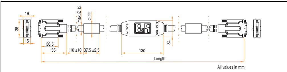
Figure 360: Dimensions - SDL flex cable with extender 5CASDL.0x00-13
