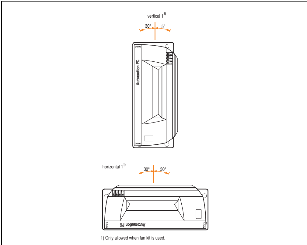
Figure 141: Mounting orientations for an APC 620 with a slide-in CD-ROM drive
