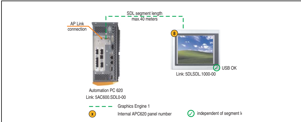
Figure 152: Configuration - One Automation Panel 900 via SDL (AP Link)
