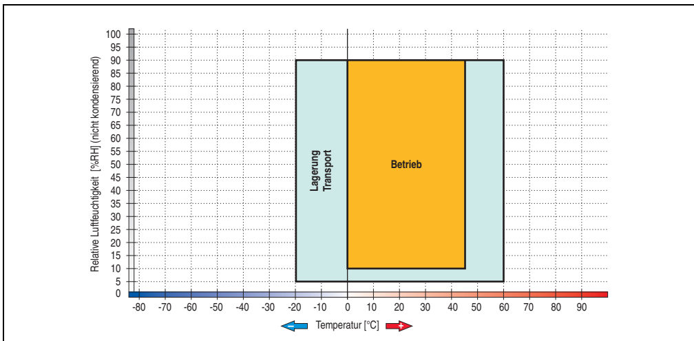
Figure 337: Temperature humidity diagram for flash drives 5MMUSB.xxxx-00
