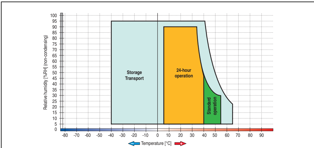
Figure 109: Temperature humidity diagram - SATA RAID hard disk 5ACPCI.RAIC-01
