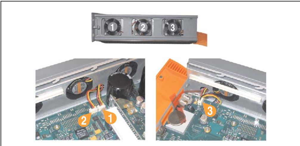
Figure 395: APC620 1PCI slot - Fan cable connection to the main board
