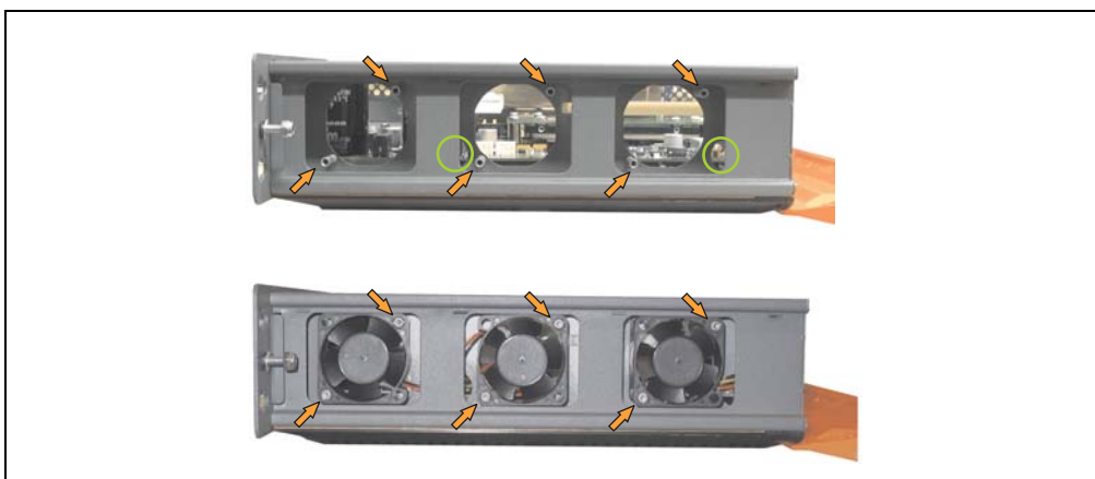
Figure 394: APC620 1PCI slot - Fan installation
