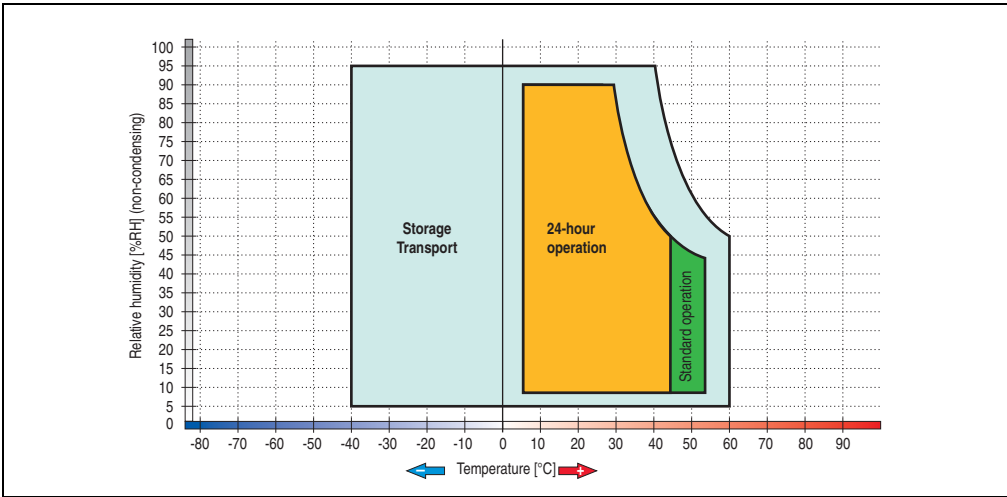
Figure 73: Temperature humidity diagram - Add-on hard disk 5AC600.HDDI-00
