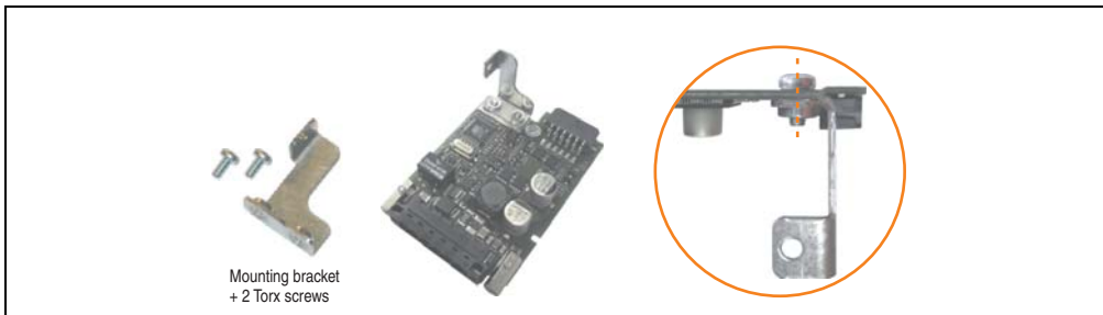
Figure 436: Install mounting bracket
