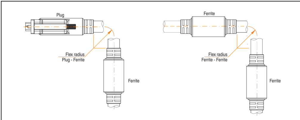
Figure 355: Flex radius specification
