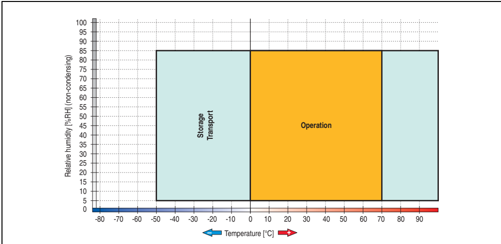
Figure 338: Temperature humidity diagram - USB flash drive - 5MMUSB.2048-01
