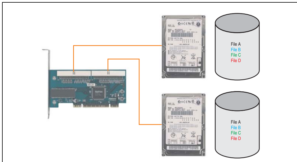
Figure 102: RAID 1 system schematic
