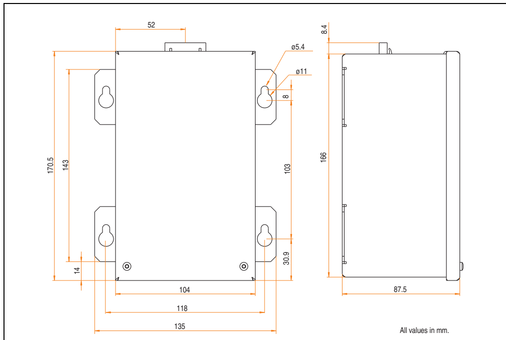
Figure 375: Dimensions - 5AC600.UPSB-00
