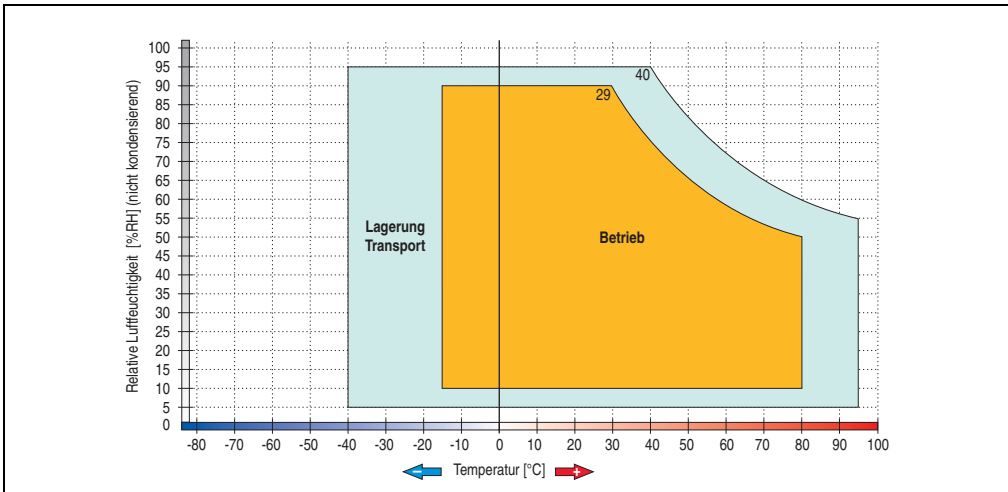
Figure 114: Temperature humidity diagram - SATA RAID hard disk 5ACPCI.RAIC-03
