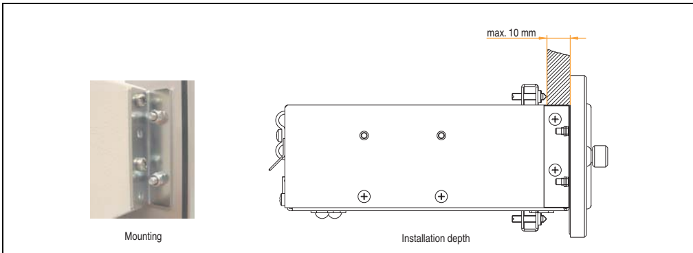
Figure 336: Front cover mounting and installation depth
