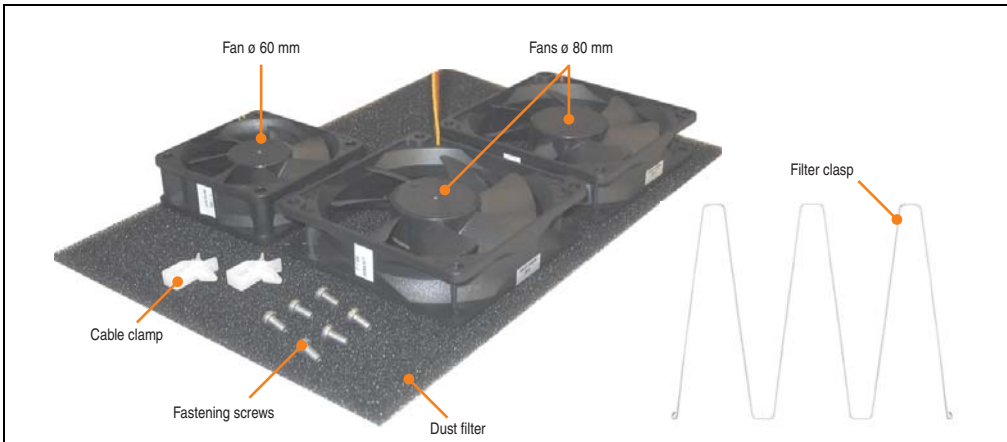
Figure 131: Fan kit - 5PC600.FA05-00
