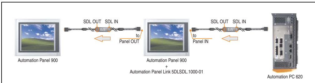
Figure 362: Example of signal direction display - SDL flex cable with extender
