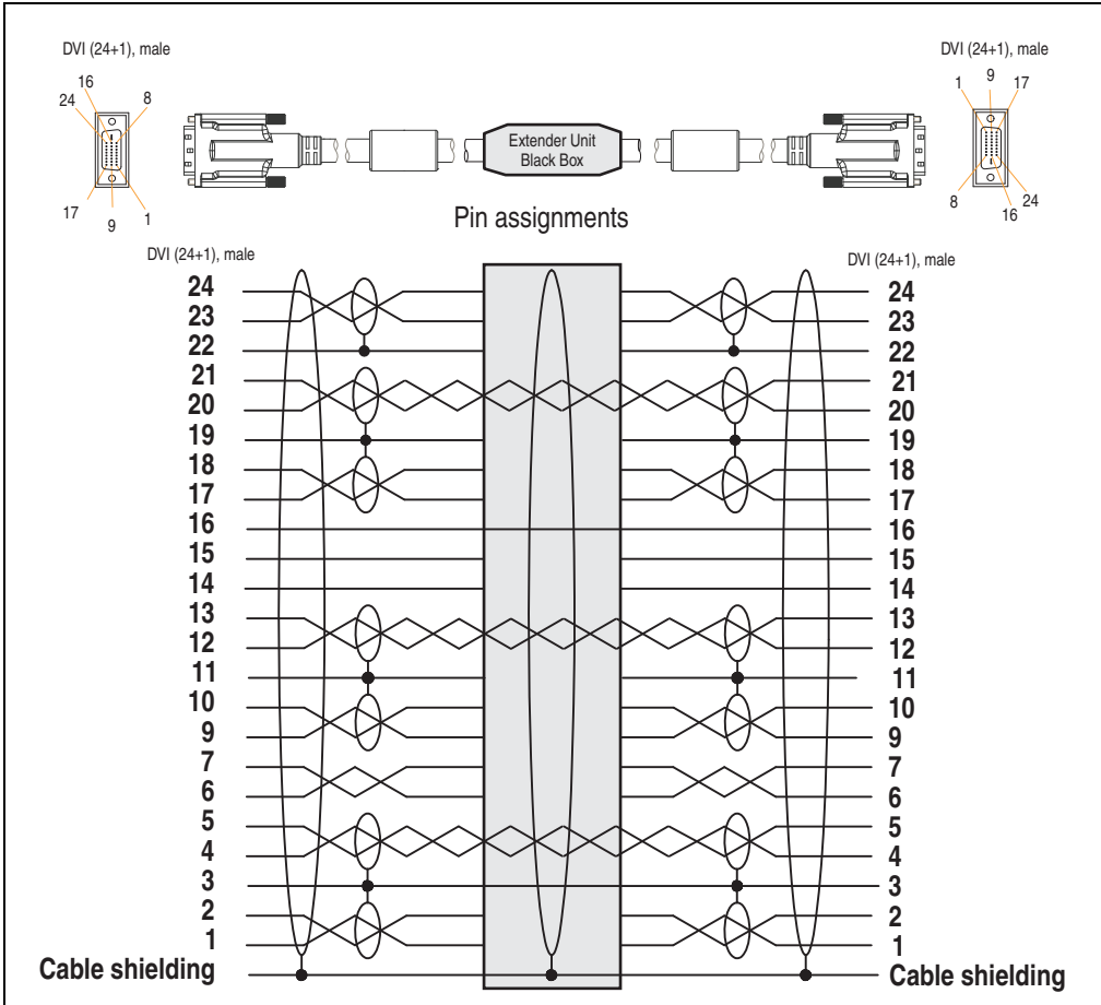
Figure 363: Pin assignments - SDL flex cable with extender 5CASDL.0x00-13
