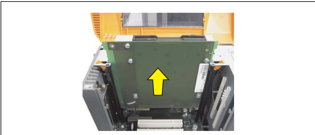
Figure 418: Removing the slide-in drive
