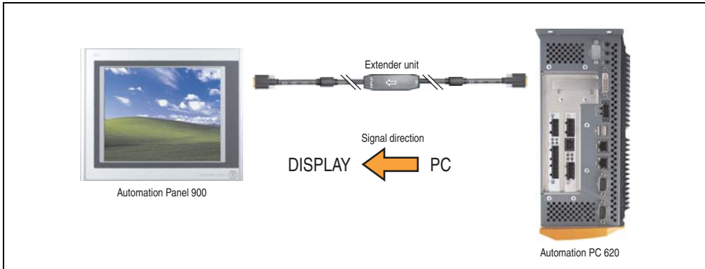
Figure 361: Example of the signal direction for the SDL flex cable with extender - APC620
