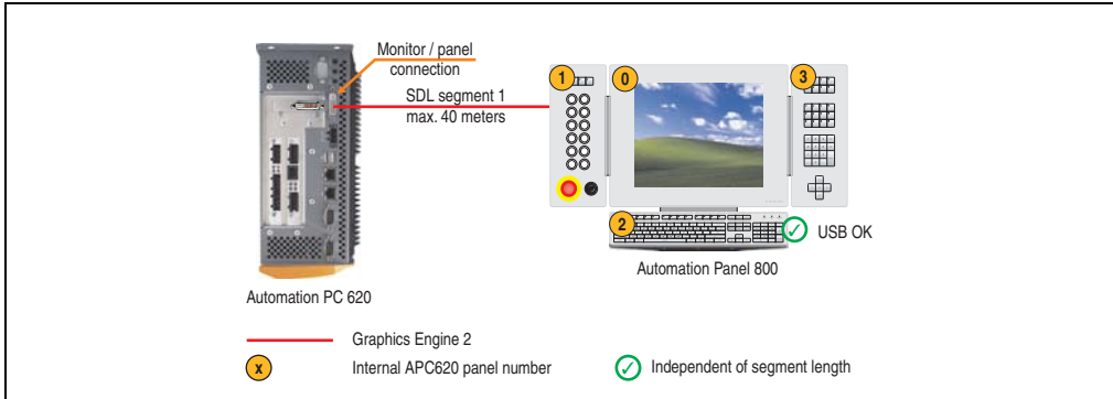
Figure 149: Configuration - An Automation Panel 800 via SDL (onboard)
