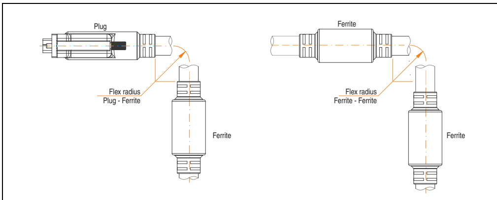
Figure 348: Flex radius specification
