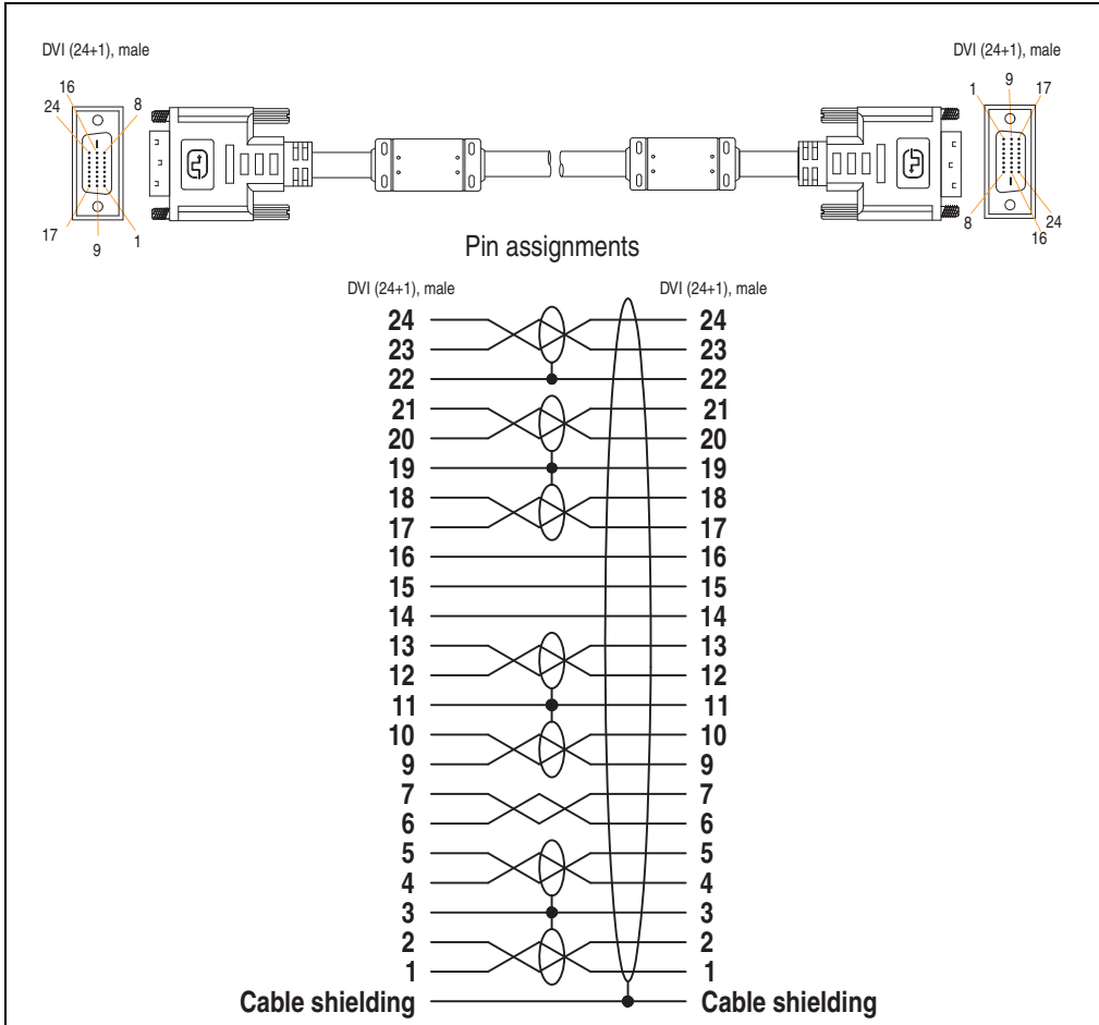
Figure 346: Pin assignments - SDL cable 5CASDL.0xxx-00
