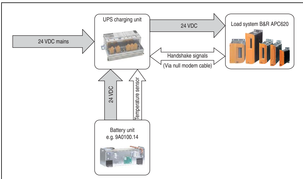
Figure 378: Block diagram of the UPS
