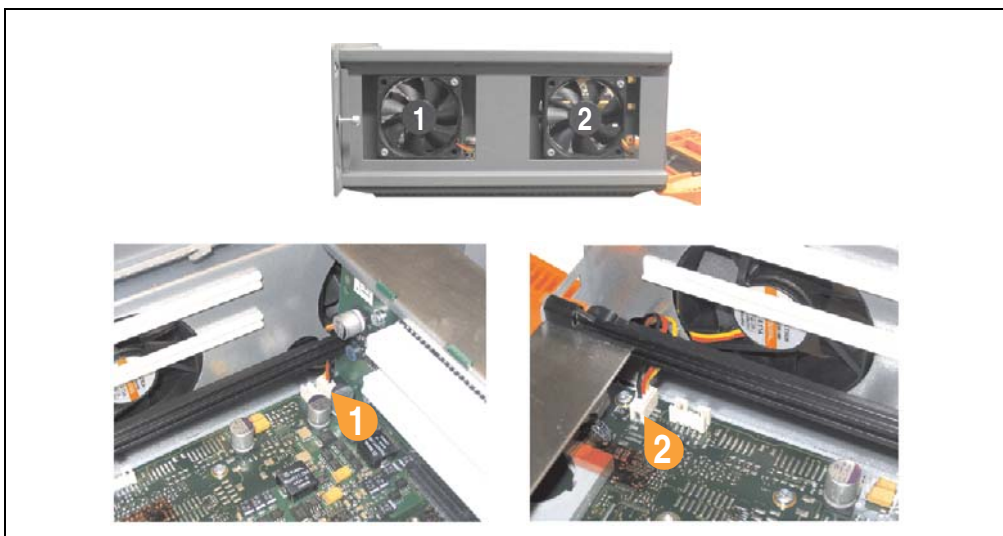
Figure 400: APC620 2PCI slots - Fan cable connection to the main board
