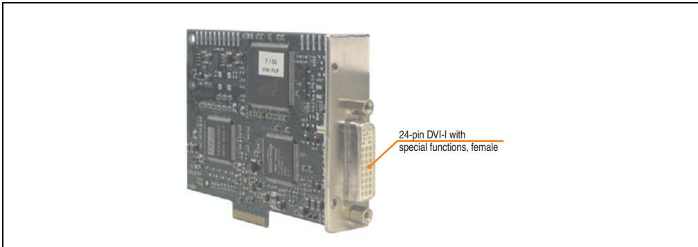
Figure 132: AP Link card
