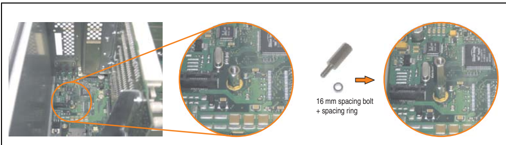
Figure 435: Screw in spacing bolt and spacing ring
