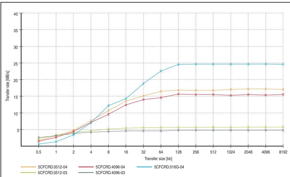
Figure 311: ATTO disk benchmark v2.34 comparison (writing)
