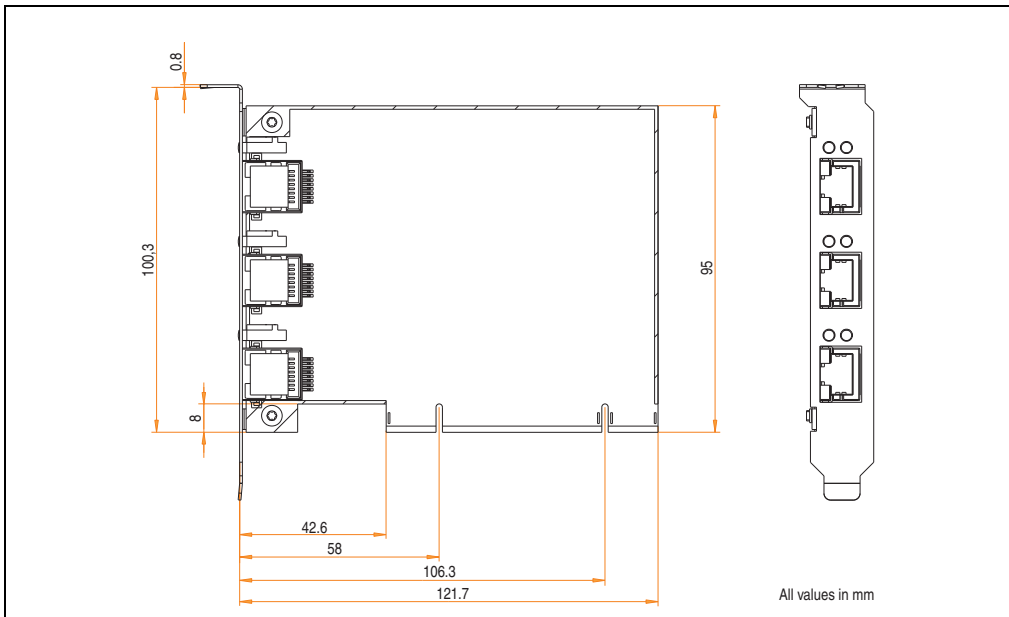
Figure 382: Dimensions - 5ACPCI.ETH3-01
