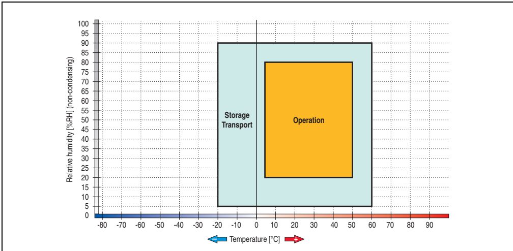
Figure 95: Temperature humidity diagram - Slide-in USB diskette drive 5AC600.FDDS-00
