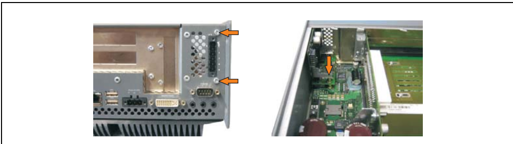
Figure 449: Install UPS module
