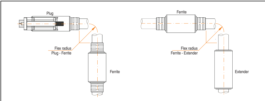
Figure 359: Flex radius specification
