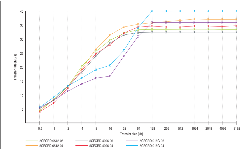
Figure 306: ATTO Benchmark v2.34 comparison when reading - 5CFCRD.xxxx-04 with 5CFCRD.xxxx-06
