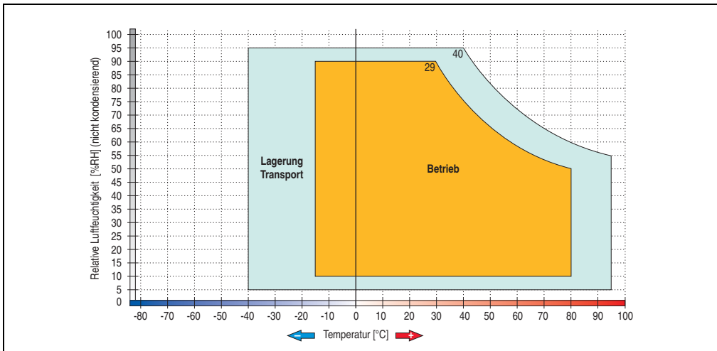
Figure 117: Temperature humidity diagram - SATA RAID hard disk 5ACPCI.RAIC-04
