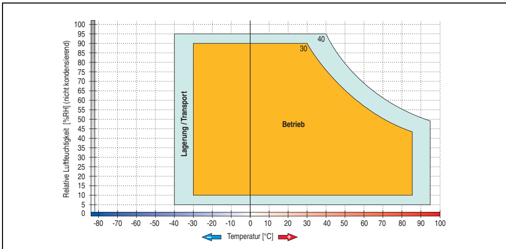
Figure 83: Temperature humidity diagram - Add-on hard disk 5AC600.HDDI-05
