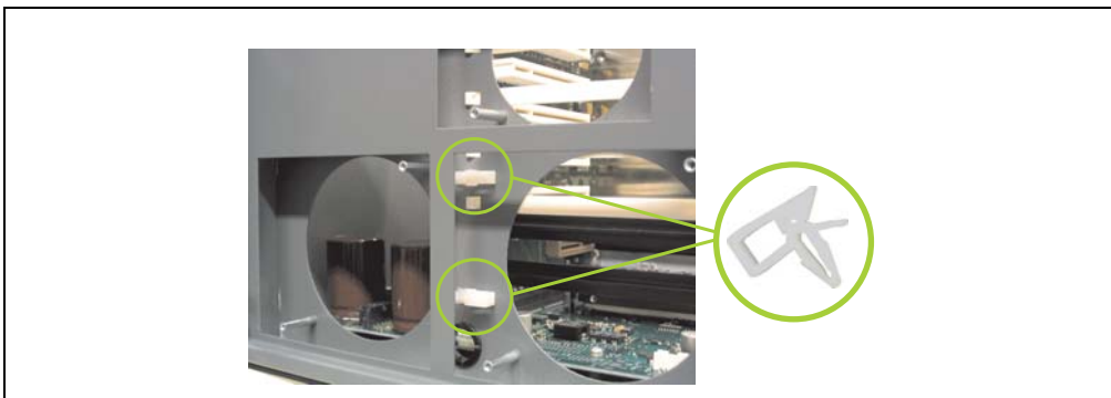
Figure 410: APC620 5PCI attach cable fasteners
