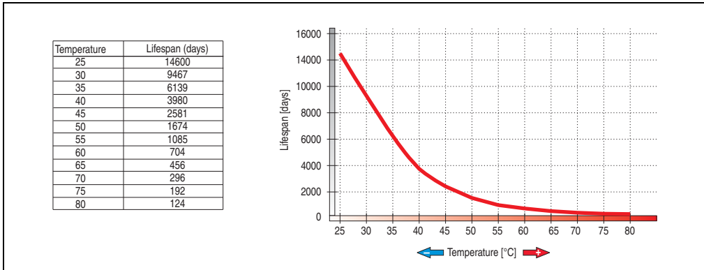
Figure 373: Temperature life span diagram
