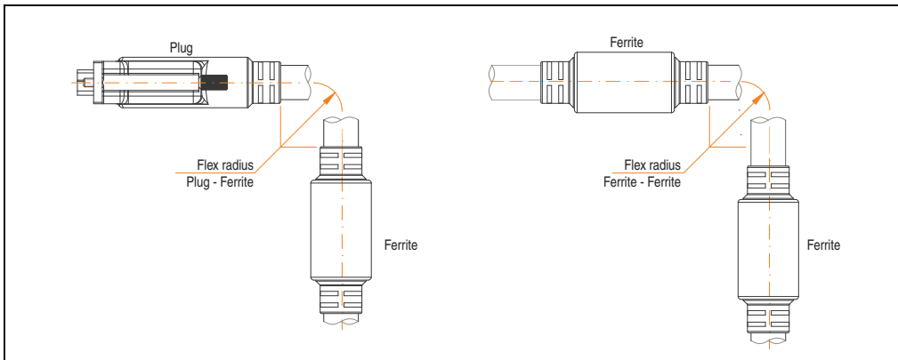
Figure 342: Flex radius specification
