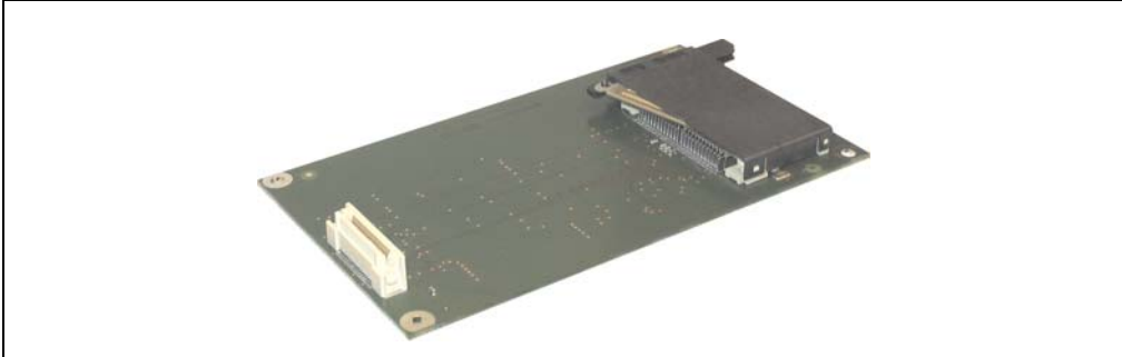
Figure 86: Add-on CompactFlash slot - 5AC600.CFSI-00
