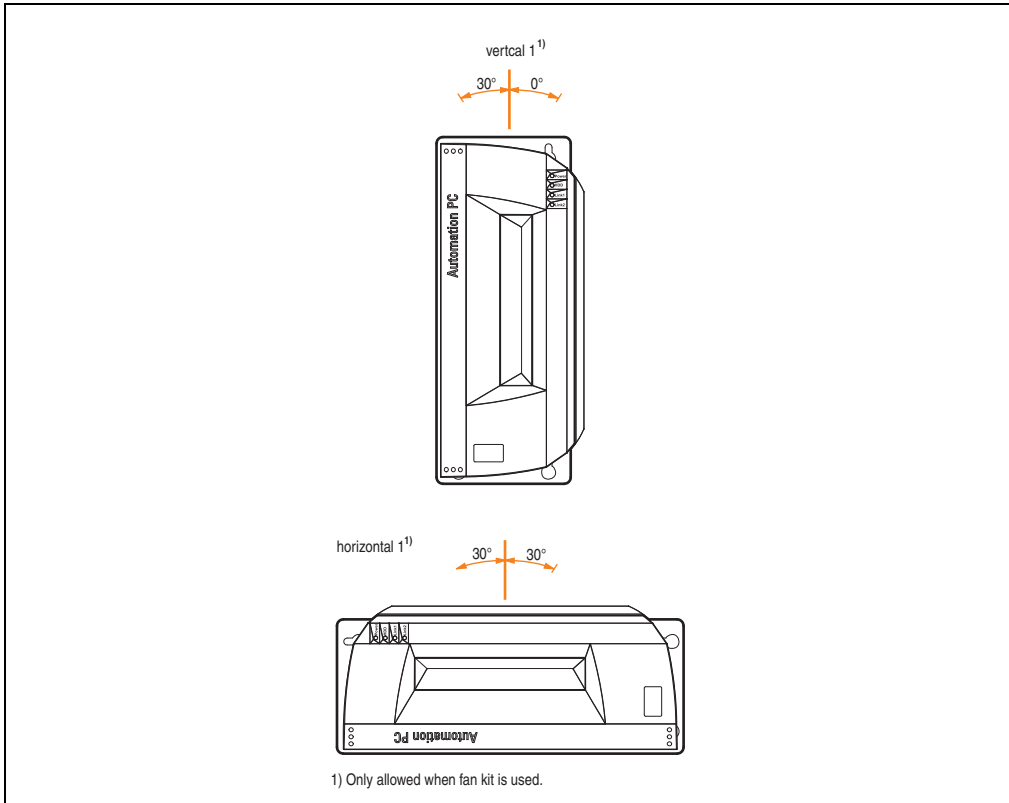
Figure 142: Mounting orientations for an APC620 with a slide-in DVD-ROM/CD-RW drive
