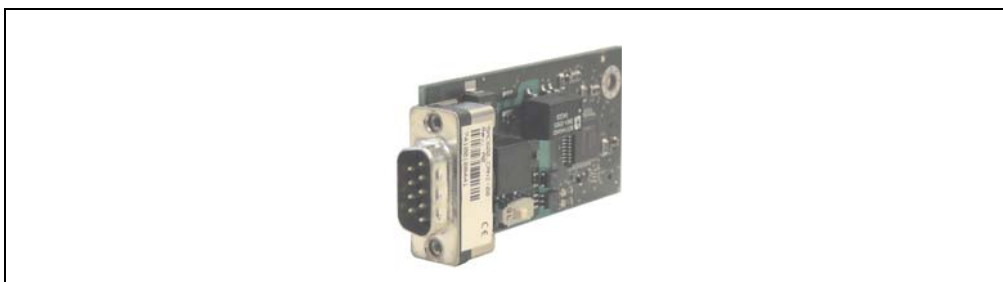
Figure 122: Add-on CAN interface - 5AC600.CANI-00
