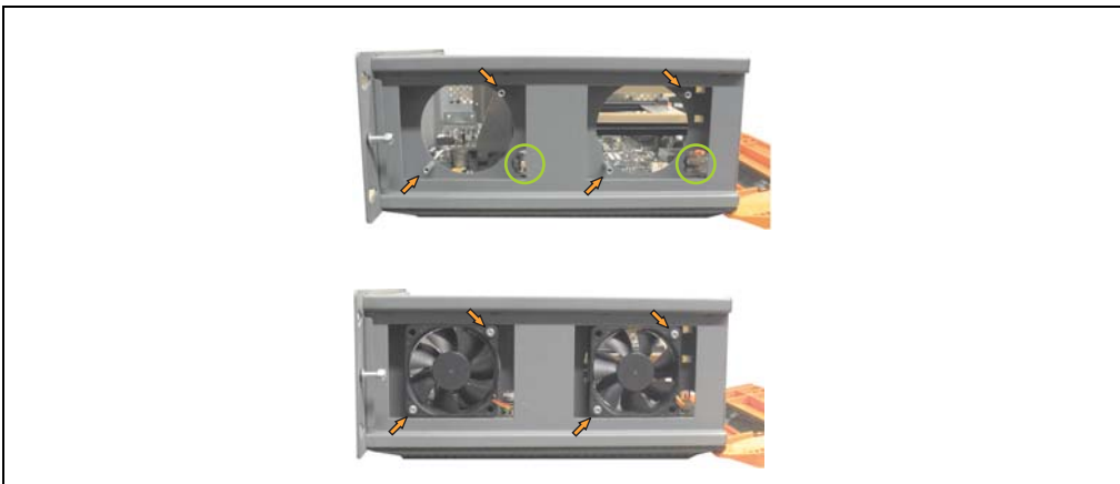
Figure 399: APC620 2PCI slots - Fan installation
