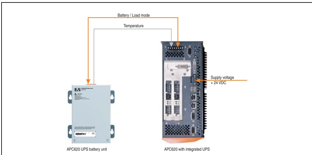
Figure 368: UPS principle
