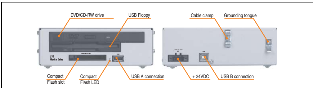
Figure 324: Interfaces for USB Media Drive 5MD900.USB2-00
