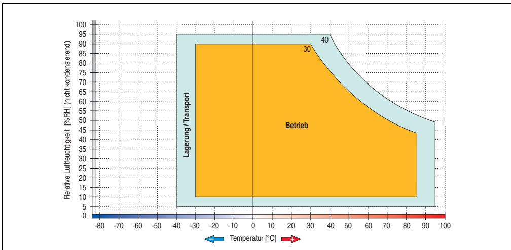
Figure 101: Temperature humidity diagram - Slide-in hard disk 5AC600.HDDS-02
