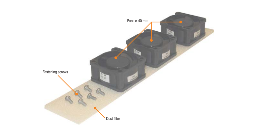
Figure 128: Fan kit - 5PC600.FA01-00
