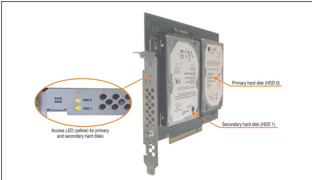
Figure 108: PCI SATA RAID controller - 5ACPCI.RAIC-01
