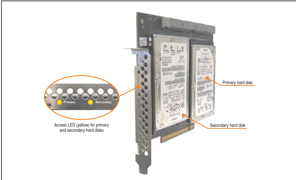
Figure 104: PCI RAID storage - 5ACPCI.RAIS-00
