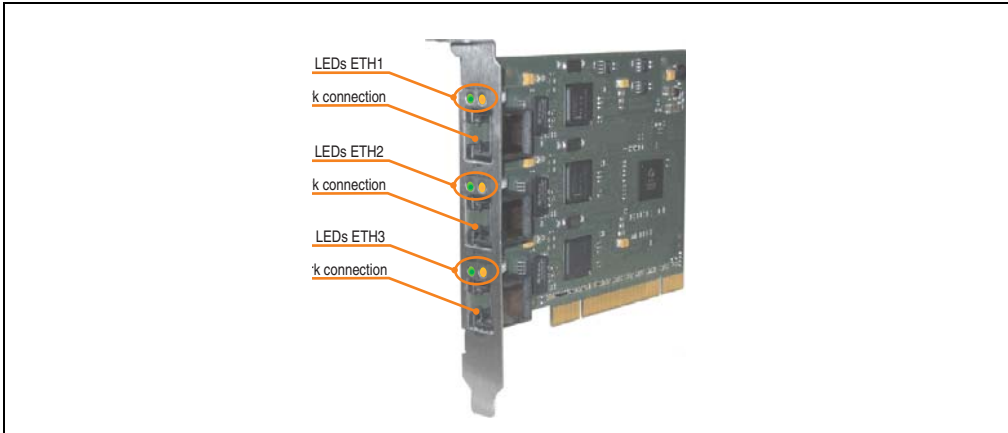
Figure 381: PCI Ethernet card 10/100 - 5ACPCI.ETH3-01
