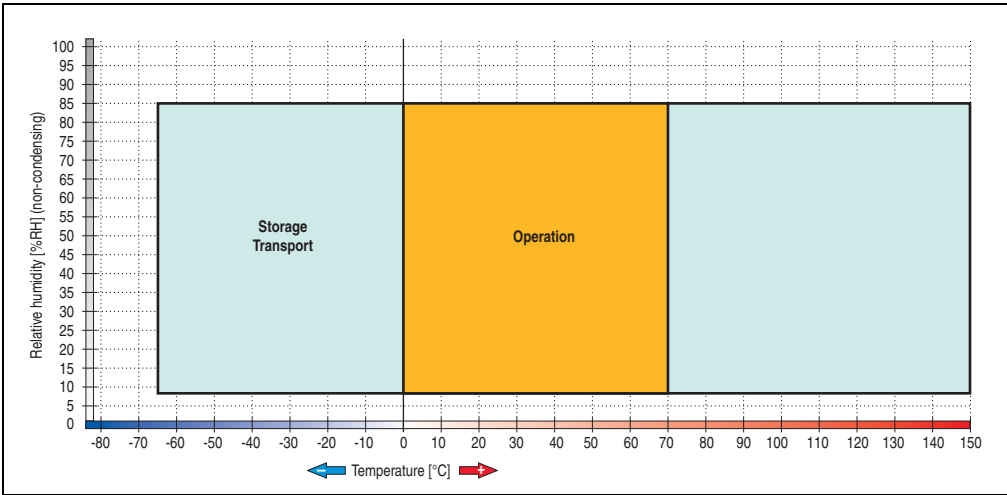
Figure 308: Temperature humidity diagram - CompactFlash cards 5CFCRD.xxxx-04
