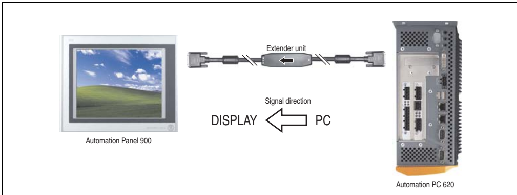
Figure 352: Example of the signal direction for the SDL cable with extender
