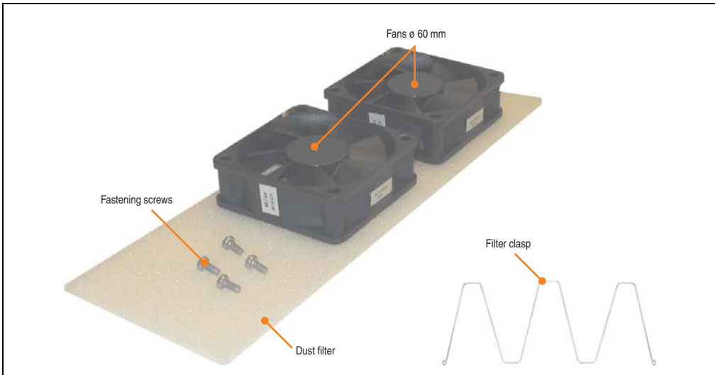
Figure 129: Fan kit - 5PC600.FA02-00
