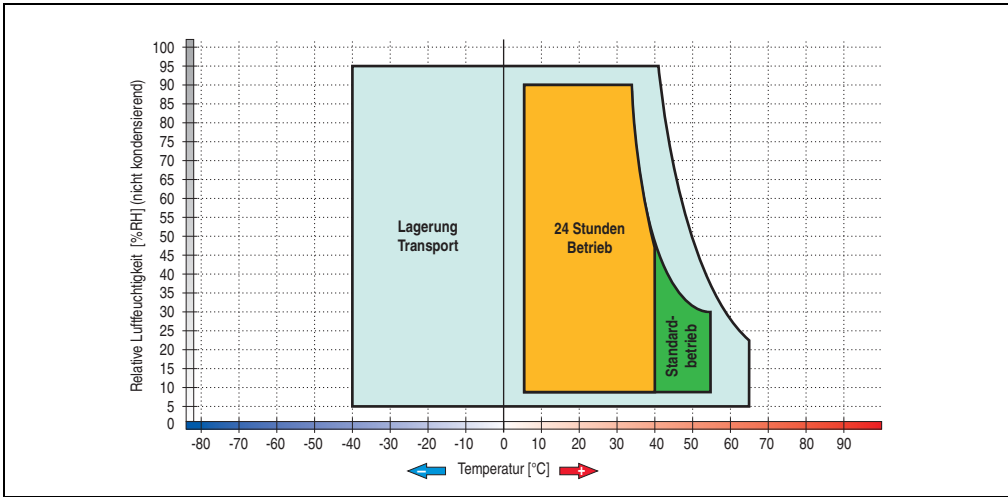
Figure 79: Temperature humidity diagram - Add-on hard disk 5AC600.HDDI-03
