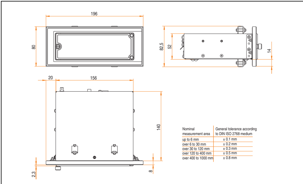
Figure 331: Dimensions - USB Media Drive with front cover
