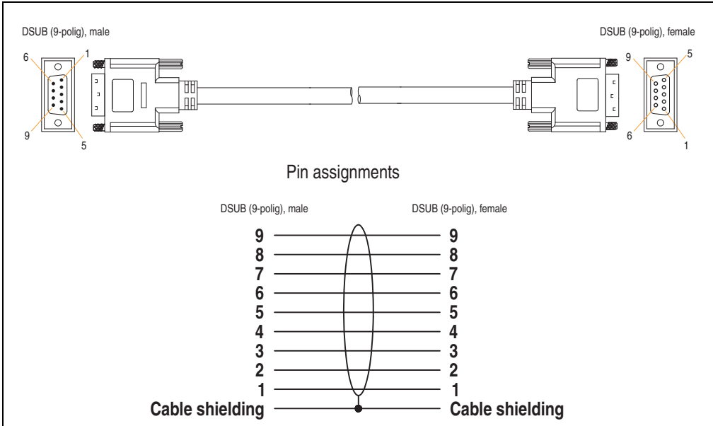
Figure 365: Pin assignments - RS232 cable
