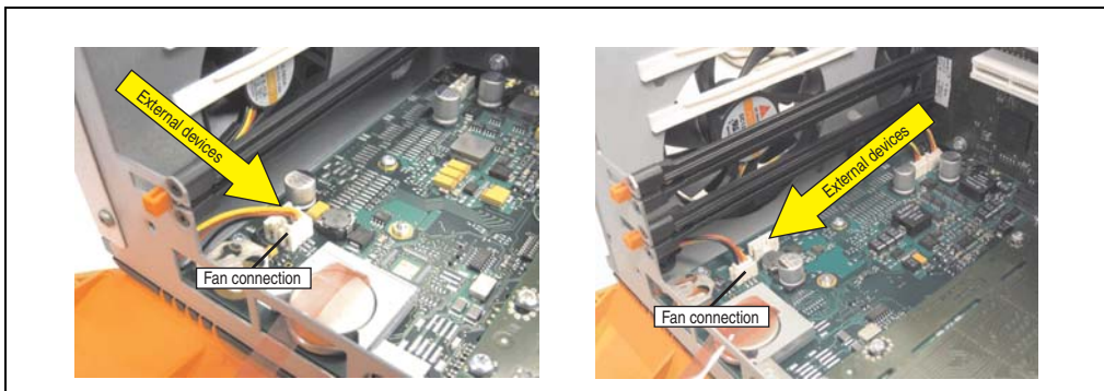
Figure 471: Connector location for external devices
