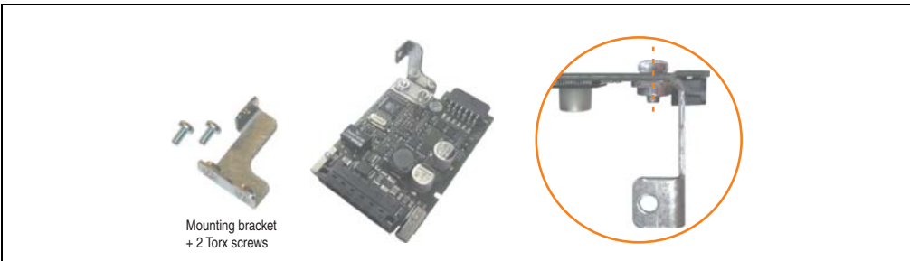
Figure 455: Install mounting bracket
