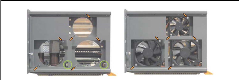
Figure 412: APC620 5PCI slot - Fan installation
