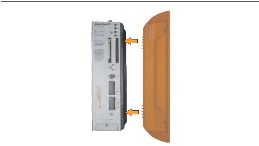
Figure 469: Attaching the front cover
