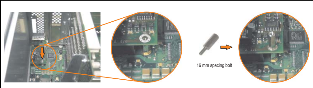
Figure 454: Screw in spacing bolt
