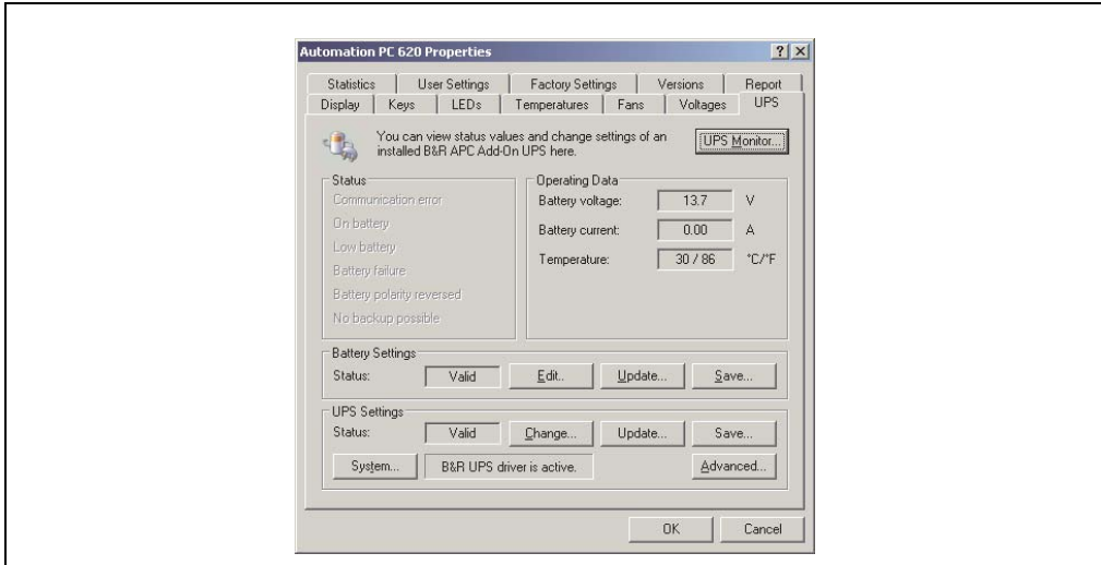
Figure 296: ADI Control Center - UPS settings
