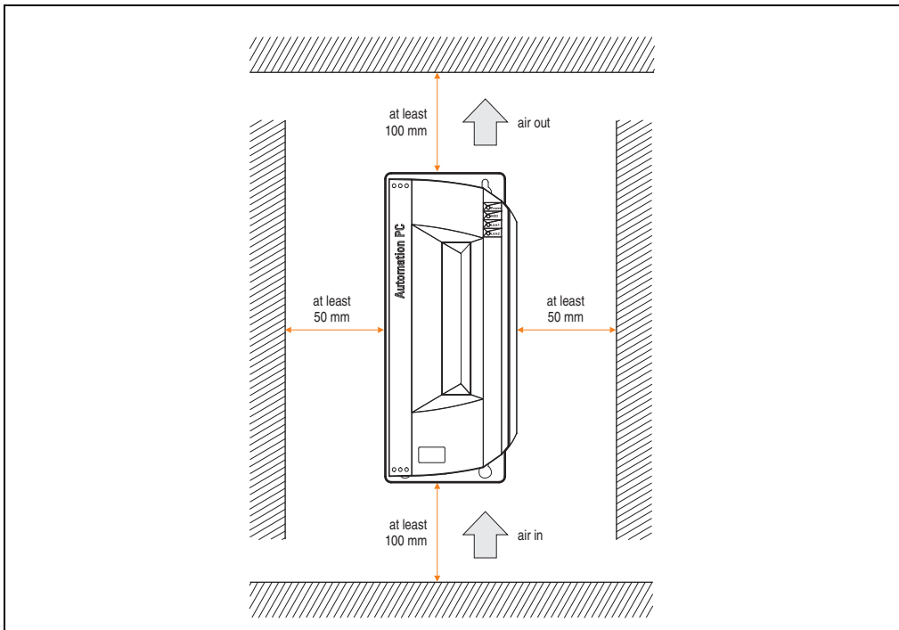
Figure 137: Air circulation spacing - Standard
