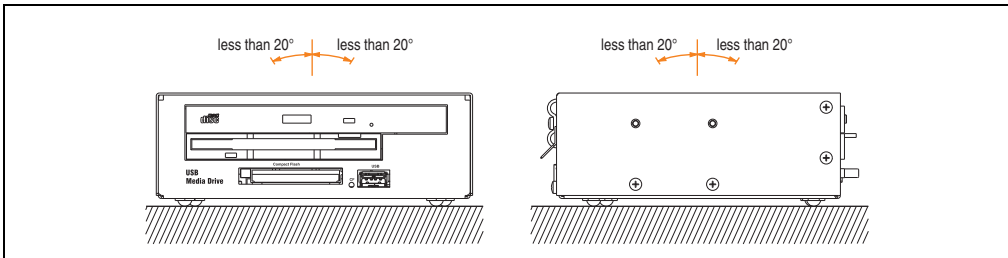
Figure 325: Mounting orientation of USB Media Drive 5MD900.USB2-00
