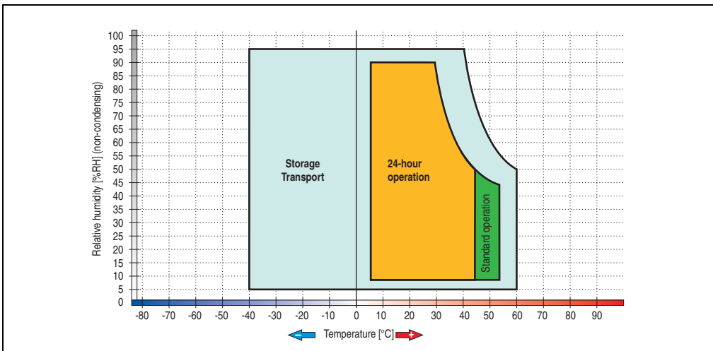
Figure 97: Temperature humidity diagram - Slide-in hard disk 5AC600.HDDS-00
