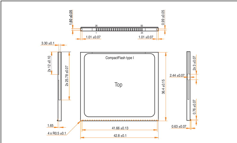
Figure 314: Dimensions - CompactFlash card Type I
