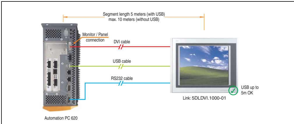
Figure 147: Configuration - One Automation Panel 900 via DVI (onboard)
