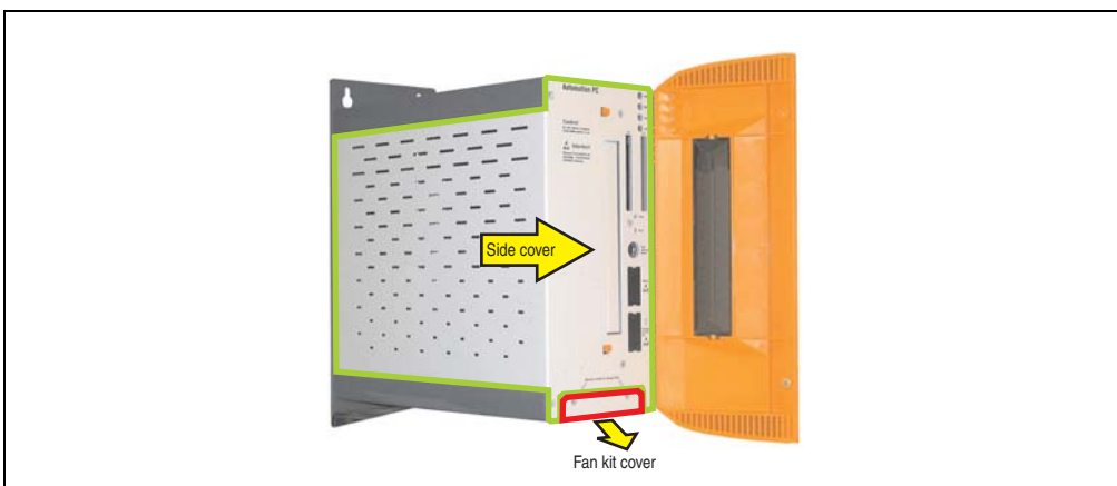
Figure 397: APC620 2PCI slots - Remove side cover and fan kit cover
