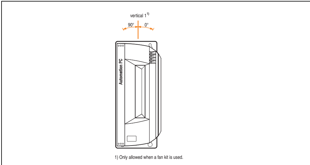
Figure 144: Mounting orientations for an APC620 with a slide-in USB FDD drive
