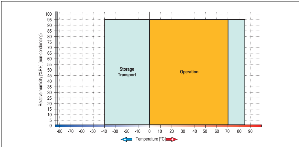
Figure 70: Temperature humidity diagram - Replacement SSD 128 GB - 5MMSSD.0128-00 ≤ D0
