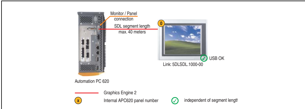
Figure 148: Configuration - An Automation Panel 900 via SDL (onboard)
