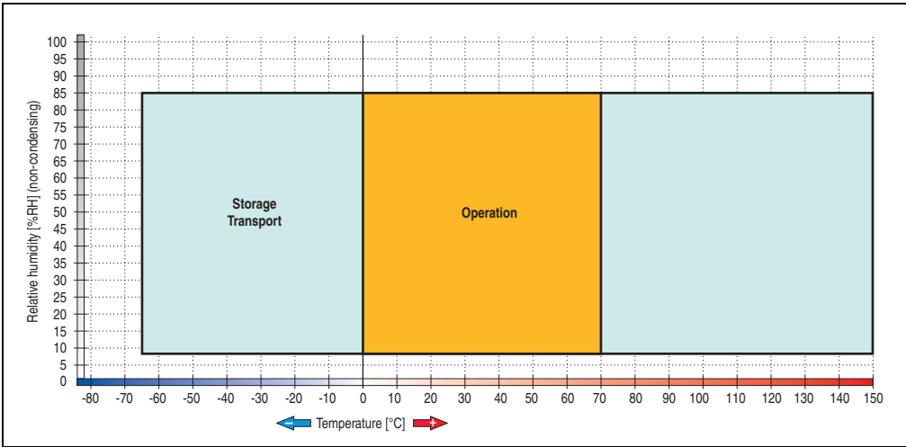
Figure 304: Temperature humidity diagram - CompactFlash cards 5CFCRD.xxxx-06
