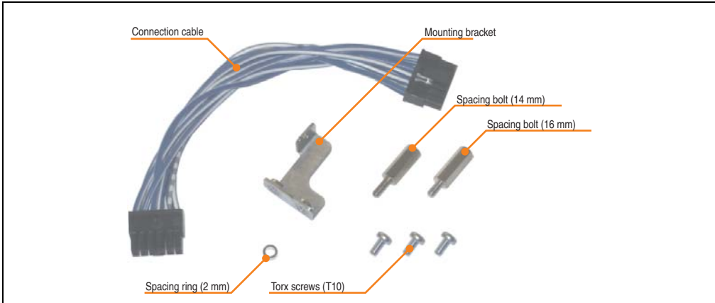
Figure 420: Add-on UPS module 5AC600.UPSI-00 - Installation materials
