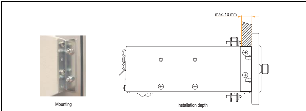
Figure 328: Front cover mounting and installation depth
