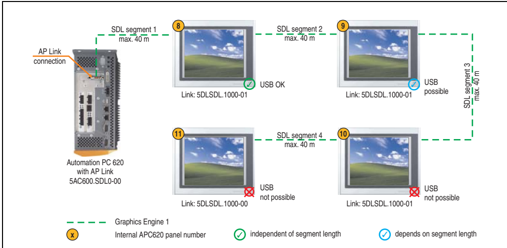
Figure 153: Configuration - 4 Automation Panel 900 units via SDL (AP Link)
