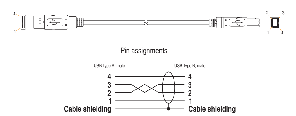
Figure 367: Pin assignments - USB cable
