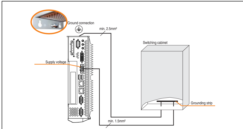
Figure 146: Grounding concept
