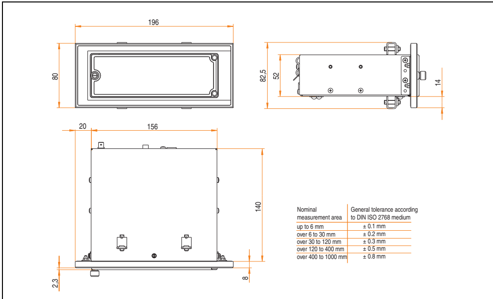
Figure 323: Dimensions - USB Media Drive with front cover
