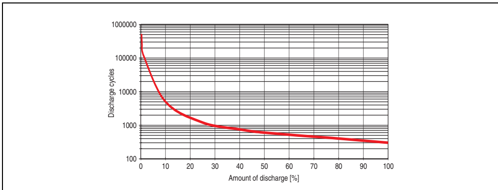
Figure 374: Deep discharge cycles
