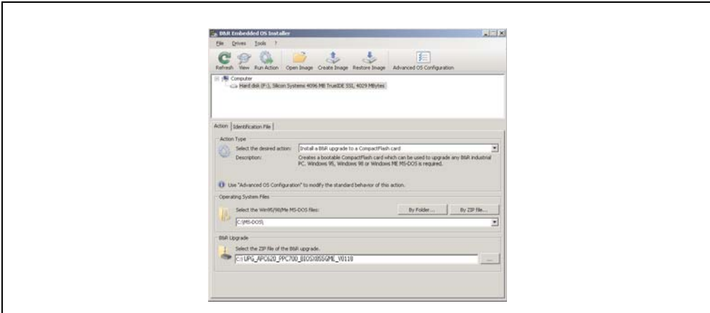
Figure 276: Creating a CompactFlash card for B&R upgrade files
