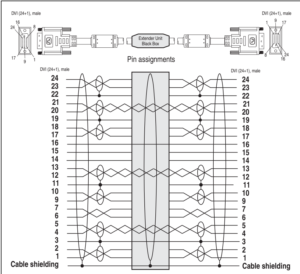
Figure 353: Pin assignments - SDL cable with extender 5CASDL.0x00-10
