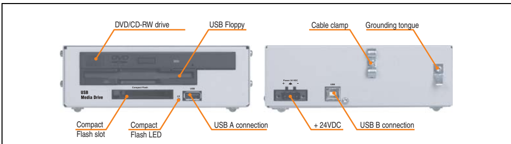
Figure 332: Interfaces - 5MD900.USB2-01
