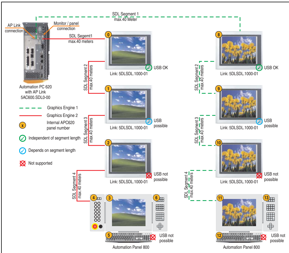
Figure 156: Configuration - Six AP900 and two AP800 devices via SDL (onboard) and SDL (AP Link)
