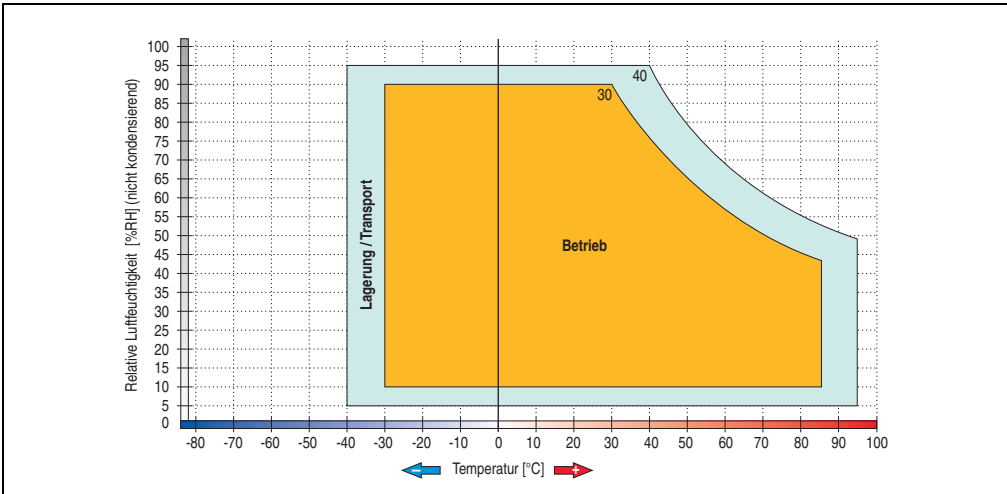
Figure 85: Temperature humidity diagram - Add-on hard disk 5AC600.HDDI-06
