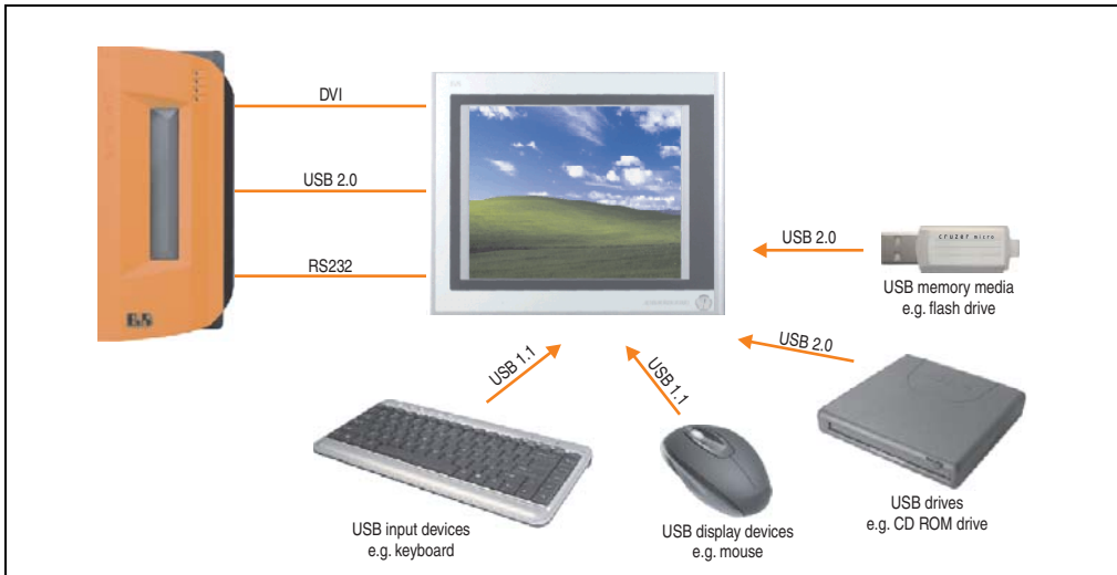
Figure 168: Remote connection of USB peripheral devices to the APC900 via DVI
