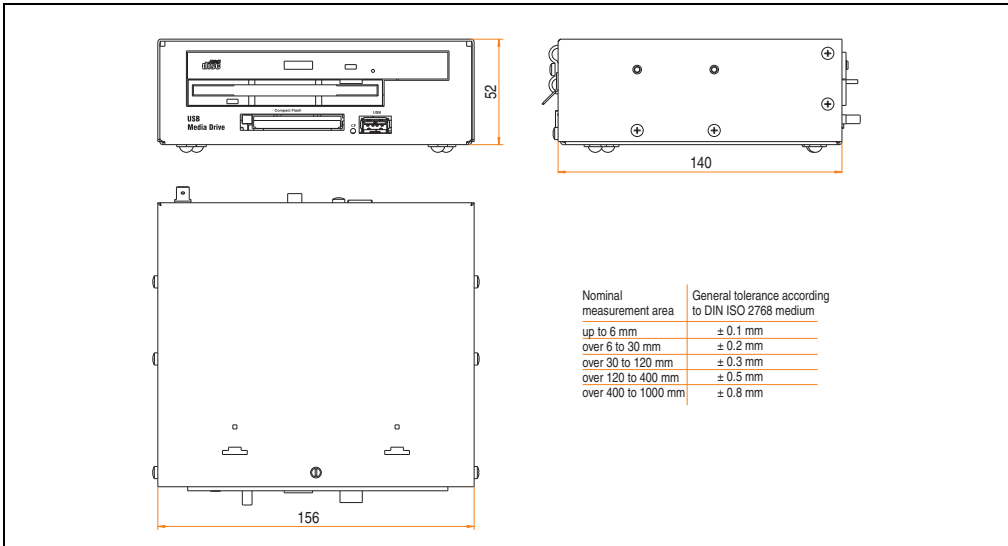
Figure 322: Dimensions for USB Media Drive 5MD900.USB2-00
