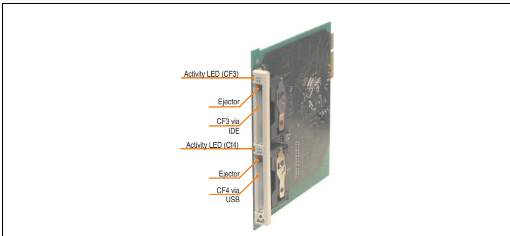
Figure 93: Slide-in CF 2-slot - 5AC600.CFSS-00
