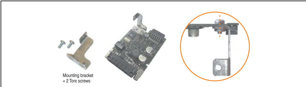
Figure 448: Install mounting bracket
