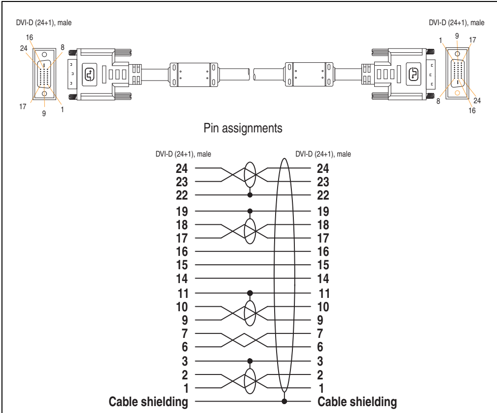
Figure 343: Pin assignments - DVI cable
