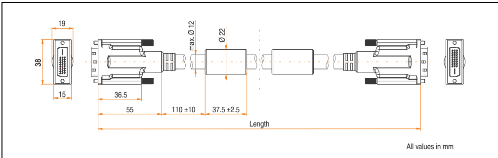
Figure 356: Dimensions - SDL cable 5CASDL.0xxx-03
