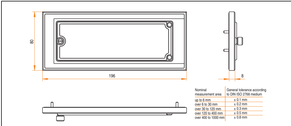
Figure 327: Dimensions - 5A5003.03
