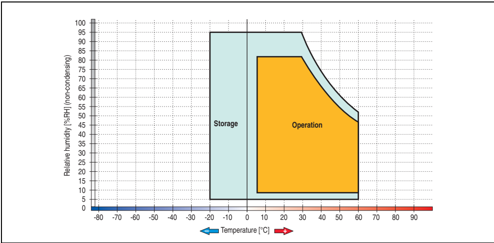
Figure 88: Temperature humidity diagram - Slide-in CD-ROM 5AC600.CDXS-00
