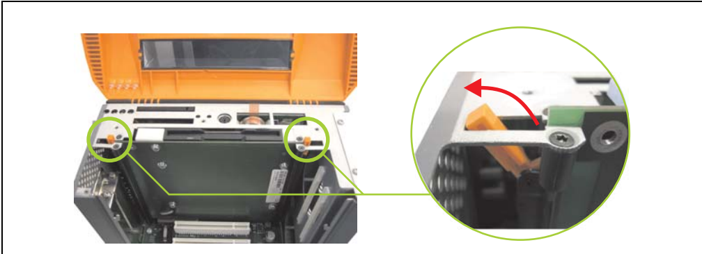
Figure 417: Release the slide-in slot releasing mechanisms
