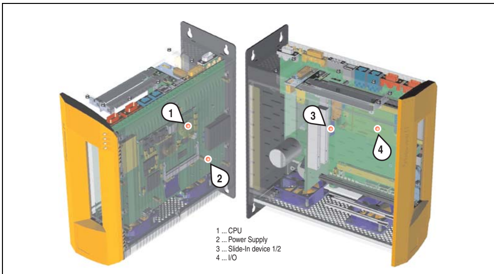
Figure 470: Temperature sensor locations
