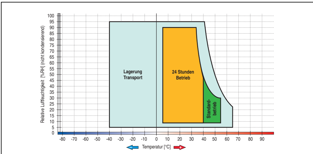
Figure 105: Temperature humidity diagram - RAID hard disk 5ACPCI.RAIS-00
