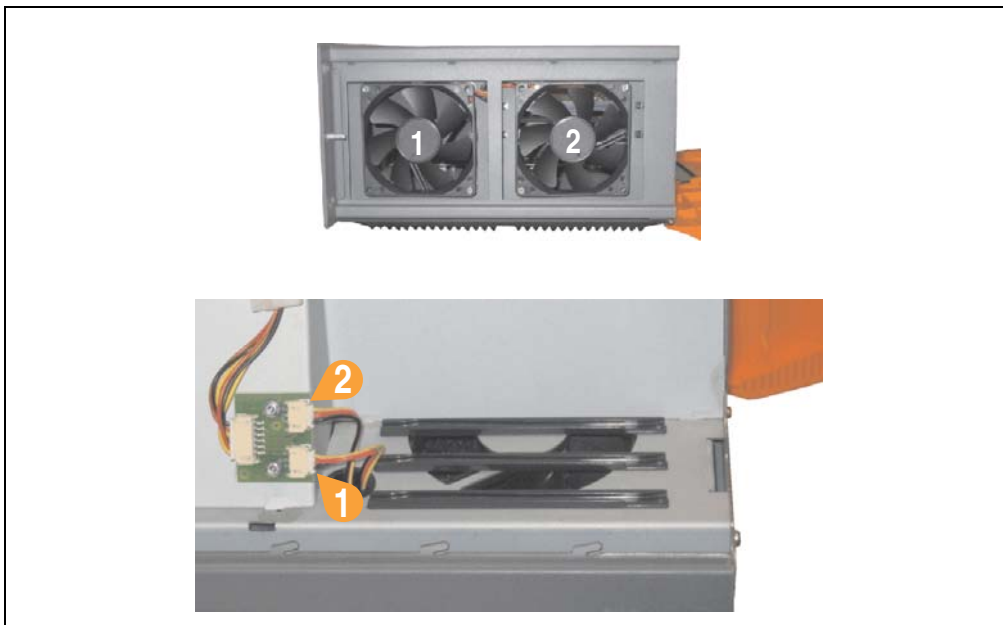
Figure 406: APC620 3PCI slot - Fan cable connection to the main board
