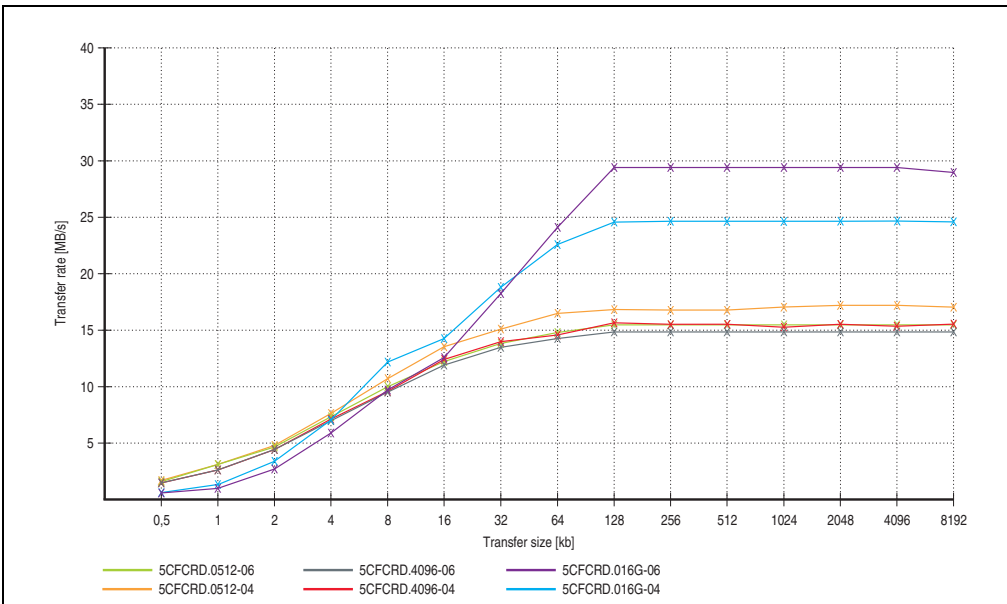
Figure 307: ATTO Benchmark v2.34 comparison when writing - 5CFCRD.xxxx-04 with 5CFCRD.xxxx-06
