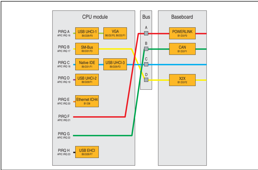
Figure 265: PCI routing with activated APIC CPU boards 855GME (XTX) on the APC620e
