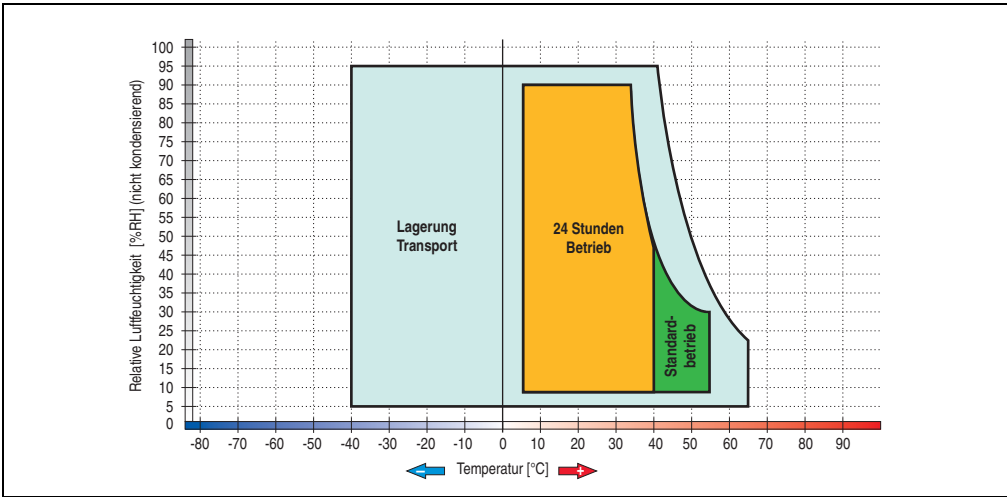
Figure 81: Temperature humidity diagram - Add-on hard disk 5AC600.HDDI-04
