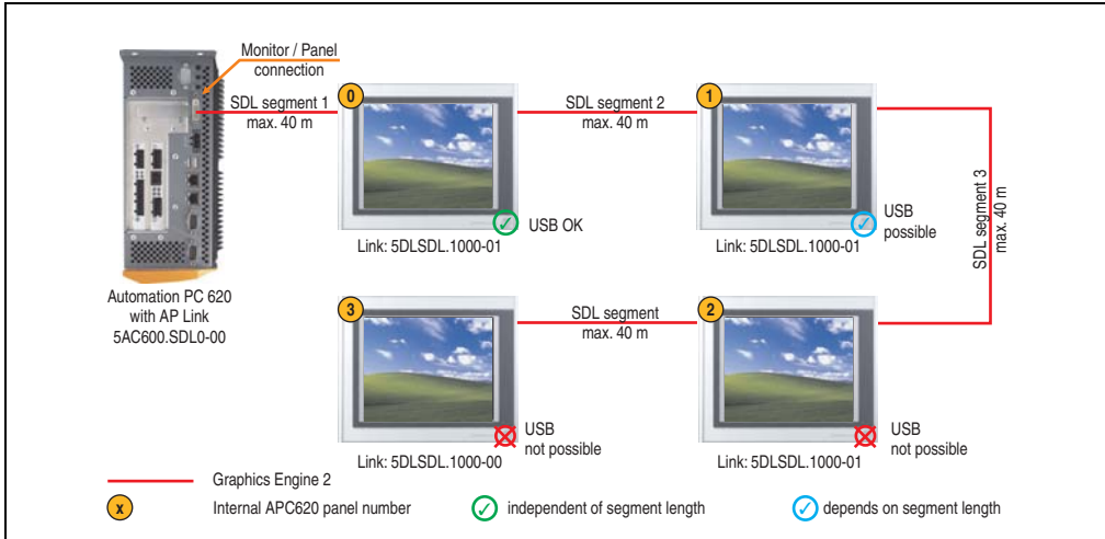
Figure 151: Configuration - Four Automation Panel 900 units via SDL (onboard)
