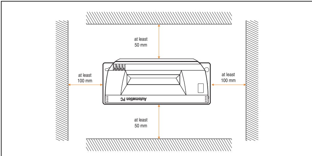
Figure 139: Optional circulation spacing
