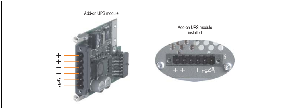
Figure 370: Add-on UPS module 5AC600.UPSI-00
