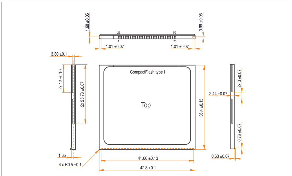
Figure 313: Dimensions - CompactFlash card Type I
