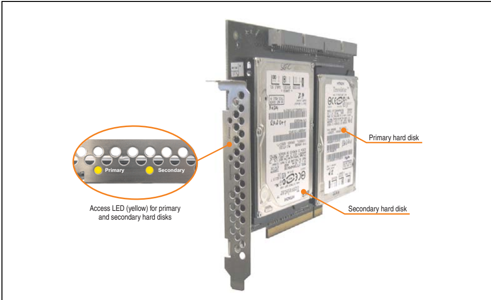
Figure 106: PCI RAID storage - 5ACPCI.RAIS-01
