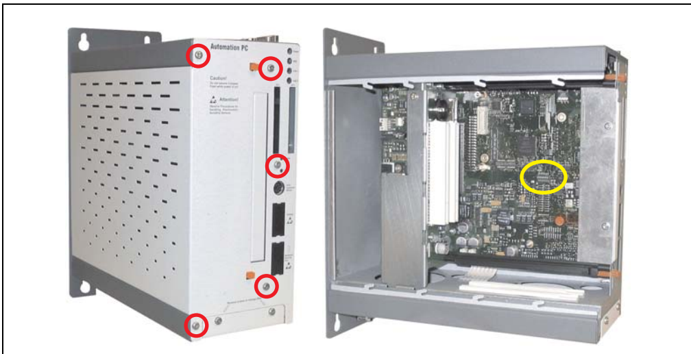
Figure 266: Location of DIP switch
