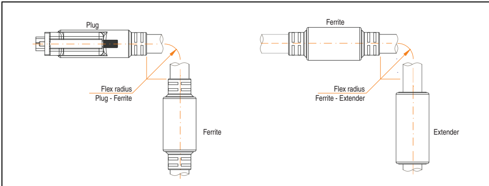
Figure 351: Flex radius specification
