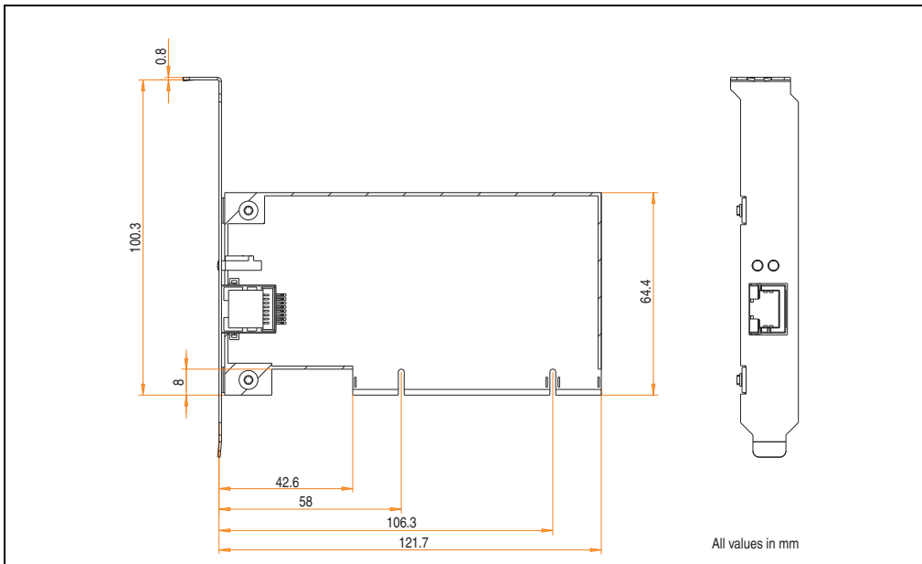
Figure 380: Dimensions - 5ACPCI.ETH1-01
