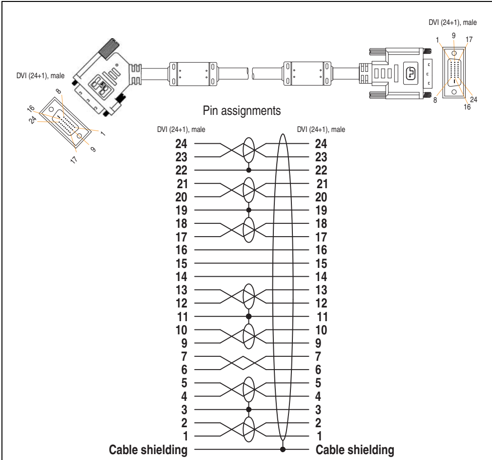
Figure 349: Pin assignments - SDL cable with 45° plug 5CASDL.0xxx-01
