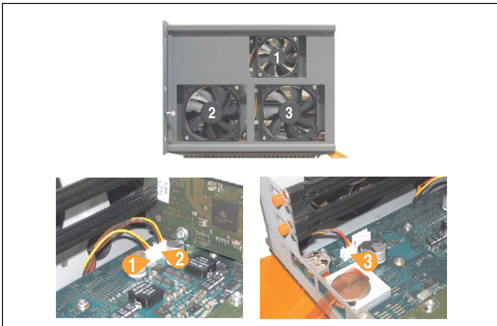
Figure 413: APC620 5PCI slot - Fan cable connection to the main board
