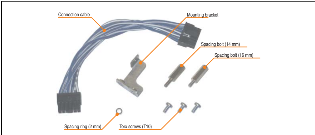
Figure 371: Add-on UPS module 5AC600.UPSI-00 - Installation materials
