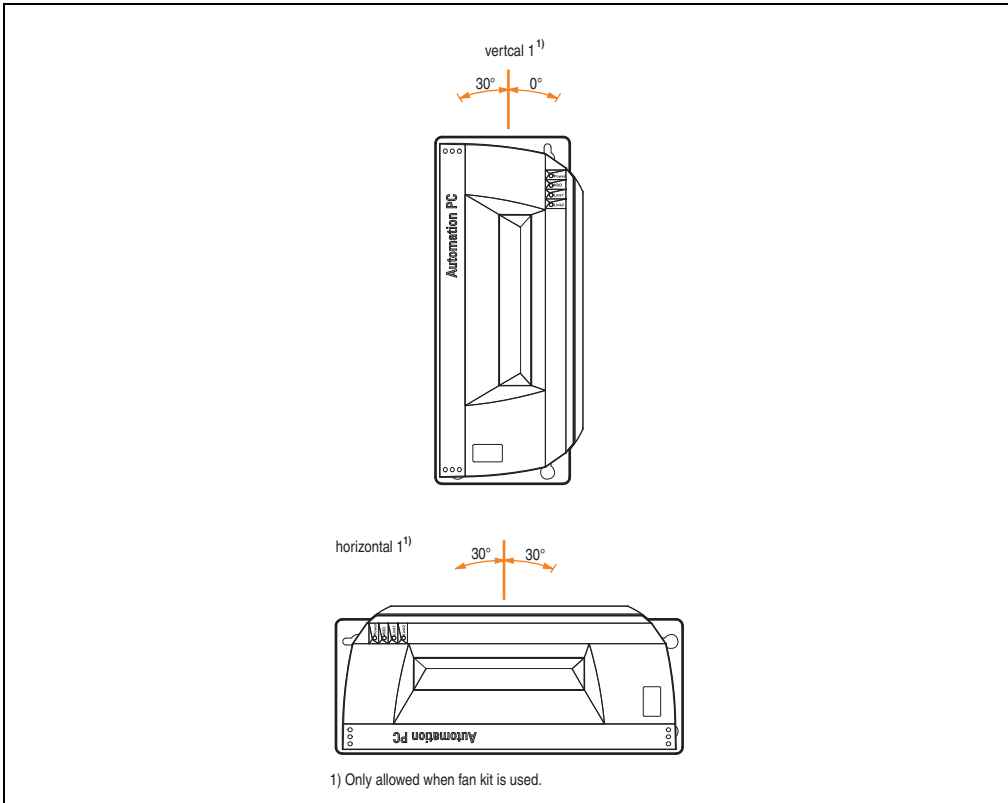
Figure 143: Mounting orientations for an APC620 with a slide-in DVD-R/RW / DVD+R/RW drive
