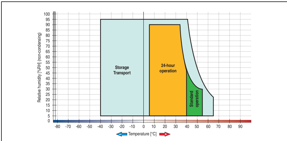
Figure 112: Temperature humidity diagram - SATA RAID hard disk 5ACPCI.RAIC-02
