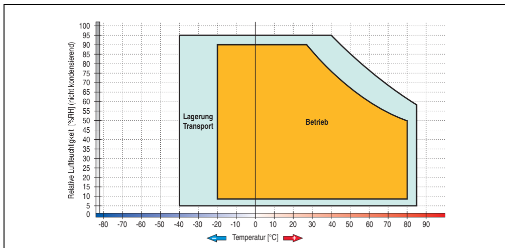
Figure 75: Temperature humidity diagram - Add-on hard disk 5AC600.HDDI-01
