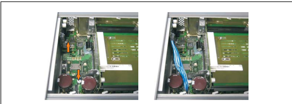
Figure 450: Plug in connection cable
