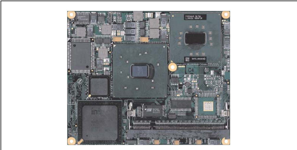
Figure 61: CPU boards 855GME (XTX)
