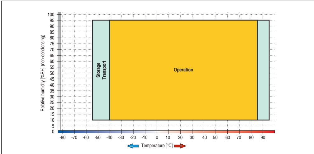
Figure 71: Temperature humidity diagram - Replacement SSD 128 GB - 5MMSSD.0128-00 ≥ E0
