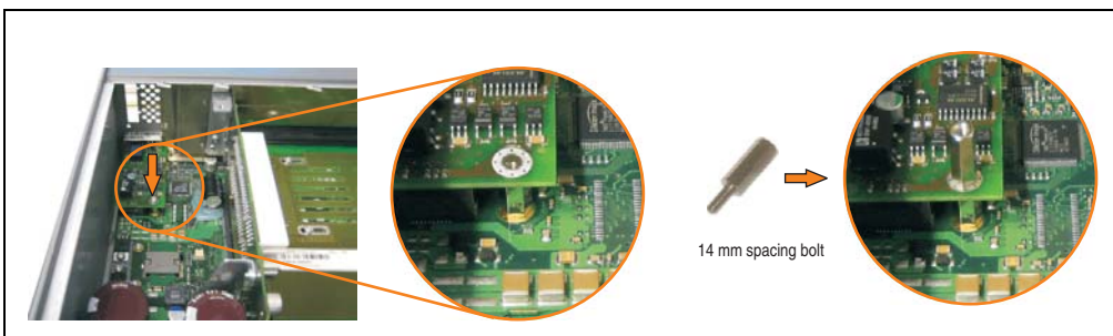
Figure 447: Screw in spacing bolt
