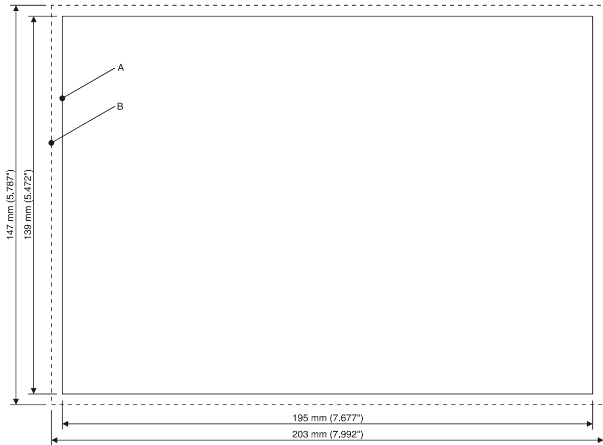
Figure 2-11 TP070ZTW / TP070GTW
