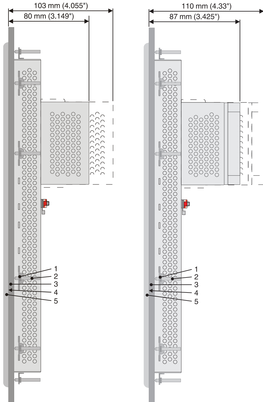
Figure 2-24 TP150ZTX / TP150GTX
