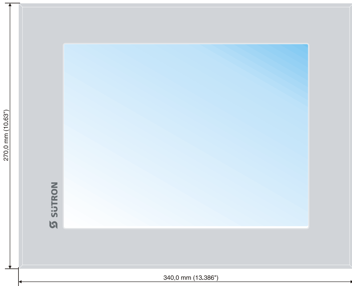
Figure 2-6 TP121ZTS / TP121GTS
