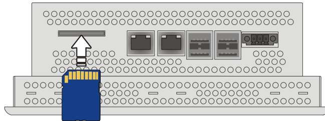
Figure 4-9 Inserting the memory card
