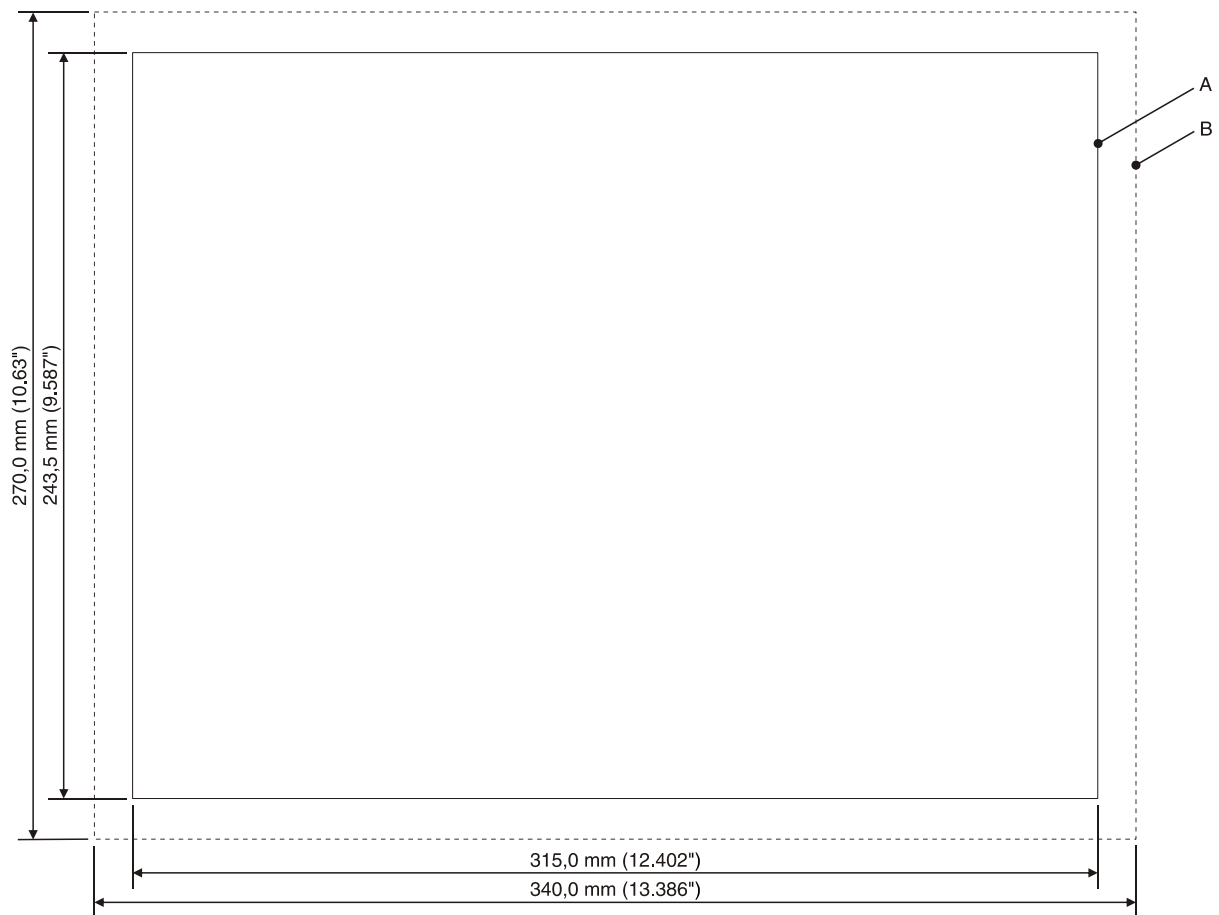
Figure 2-14 TP121ZTS / TP121GTS
