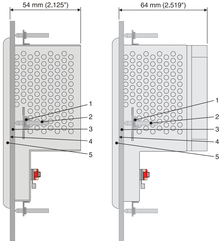
Figure 2-18 TP057ZTV / TP057GTV
