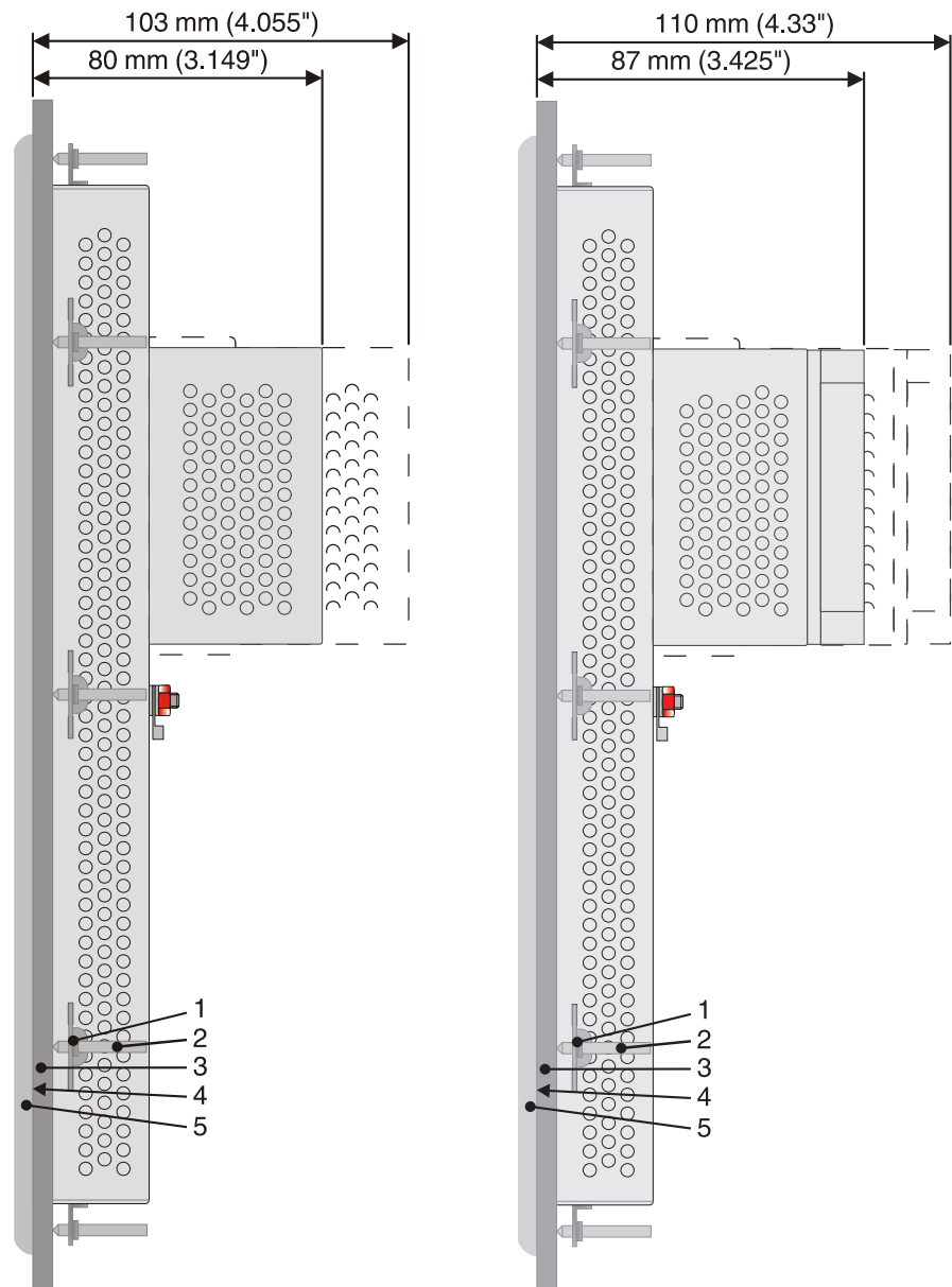
Figure 2-25 TP154ZTM / TP154GTM
