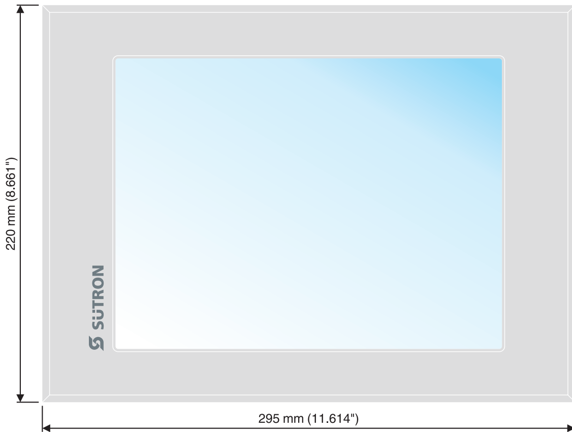
Figure 2-5 TP105ZTS / TP105GTS
