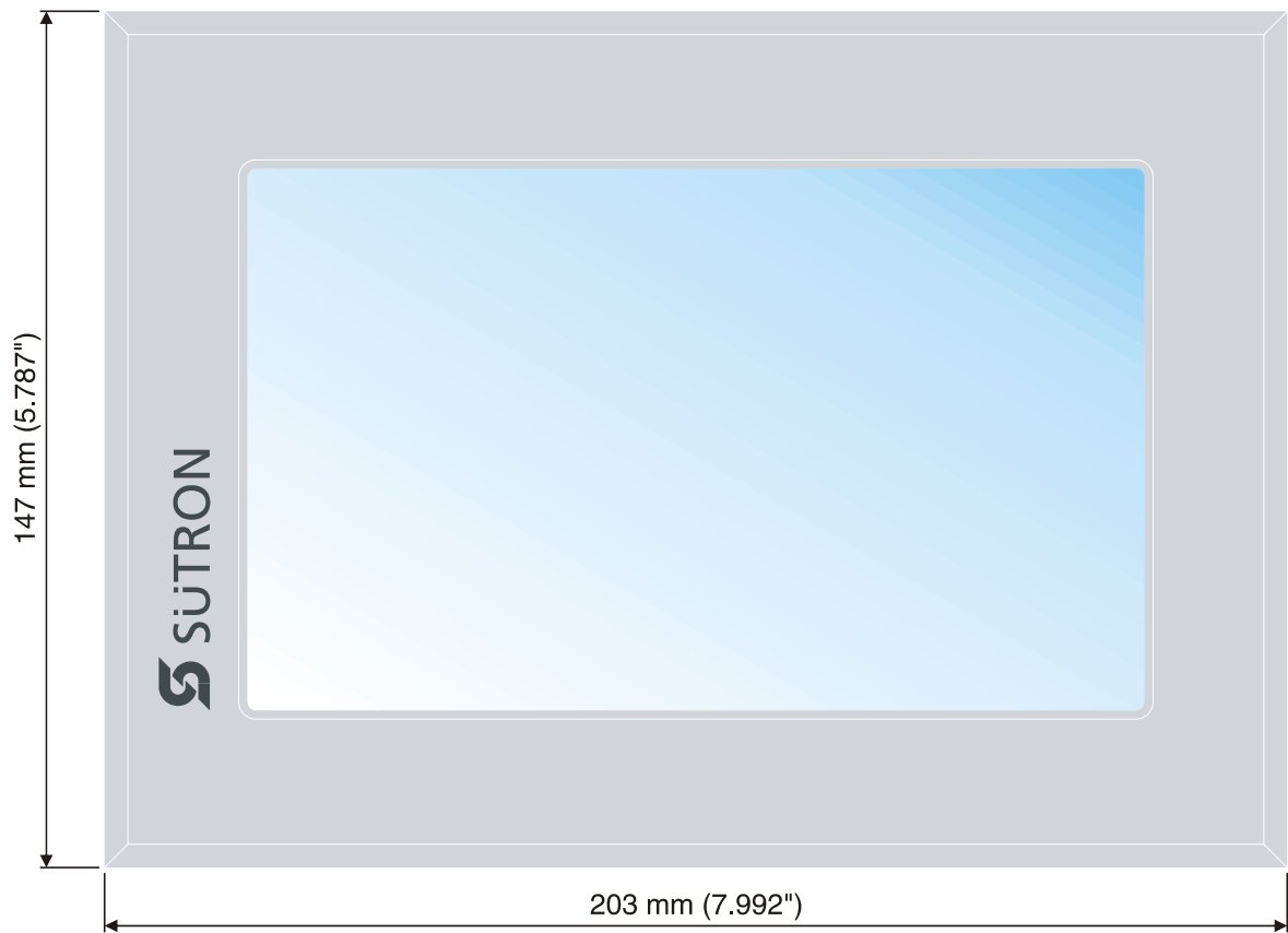
Figure 2-3 TP070ZTW / TP070GTW
