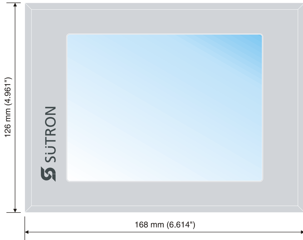
Figure 2-2 TP057ZTV / TP057GTV
