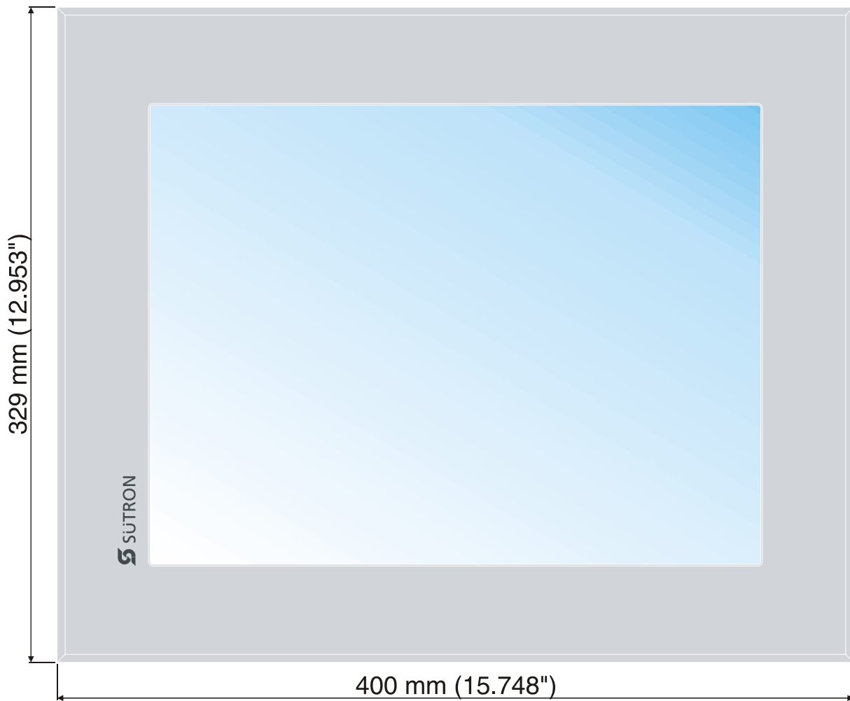
Figure 2-8 TP150ZTX / TP150GTX
