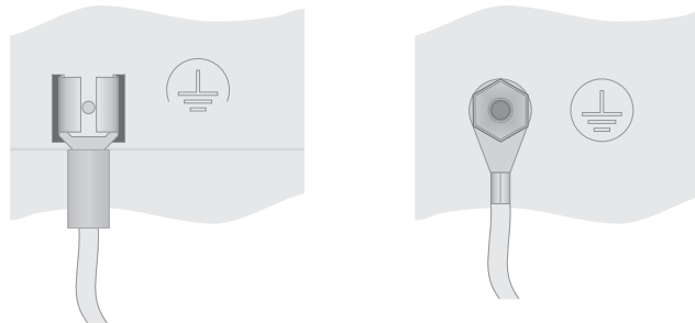
Figure 2-27 Noiseless ground / protective ground
