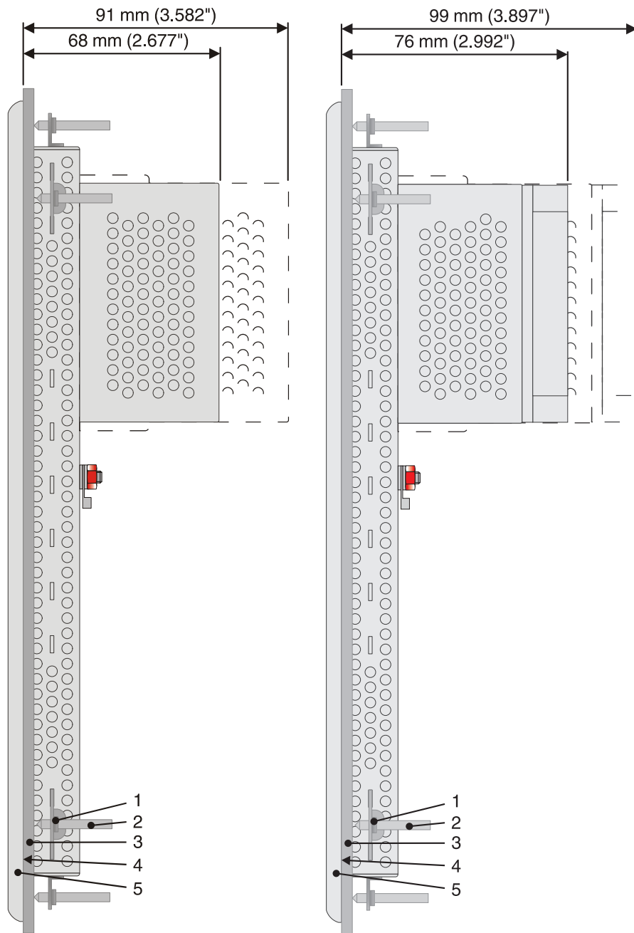
Figure 2-22 TP121ZTS / TP121GTS
