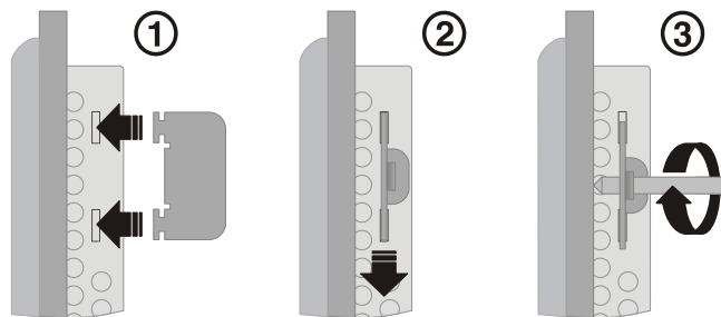
Figure 2-1 Mounting the device using a mounting bracket
