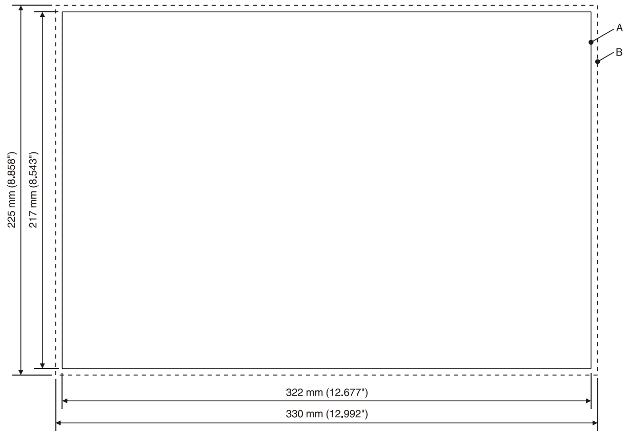
Figure 2-15 TP121ZTM / TP121GTM
