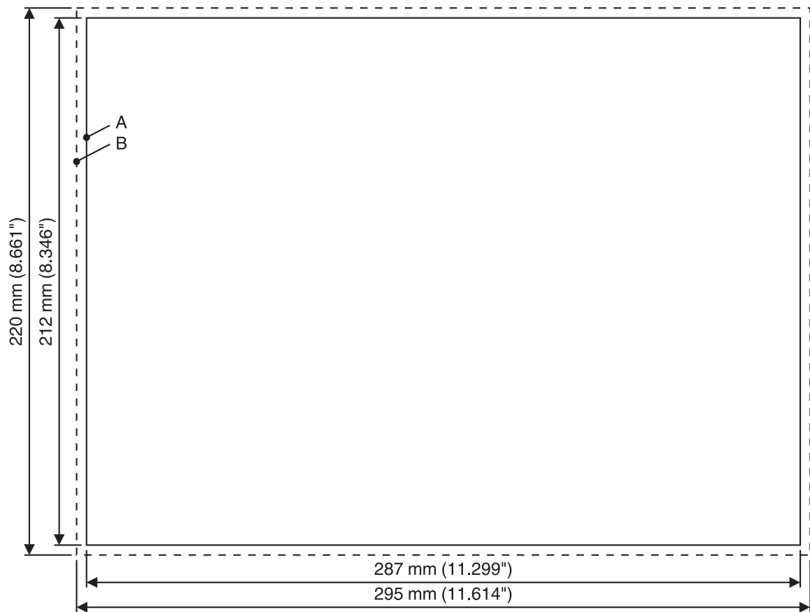
Figure 2-13 TP105ZTS / TP105GTS
