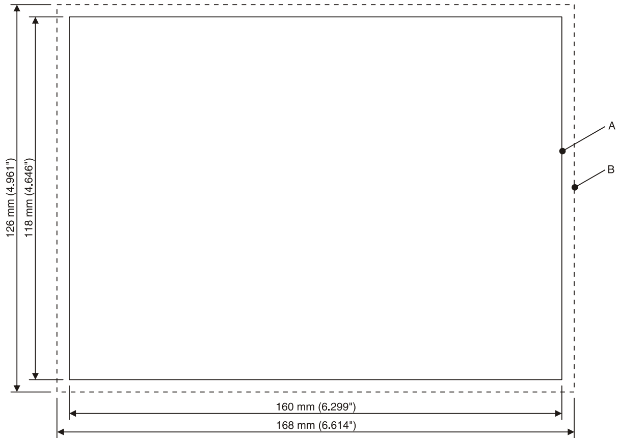
Figure 2-10 TP057ZTV / TP057GTV
