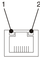
Figure 4-2 Arrangement of the Ethernet diagnostics LEDs
