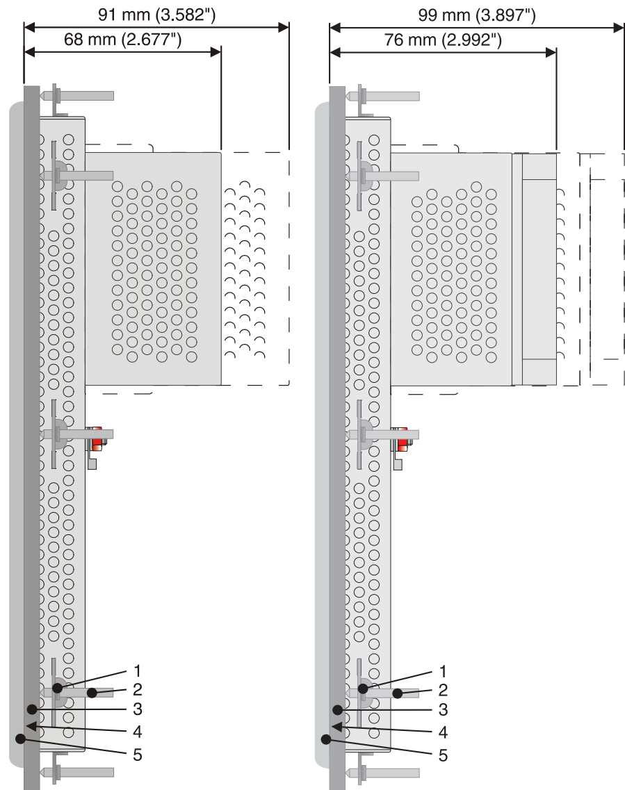
Figure 2-23 TP121ZTM / TP121GTM
