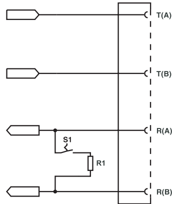
Figure 4-5 Termination possibilities RS-422 / RS-485 (intern)
