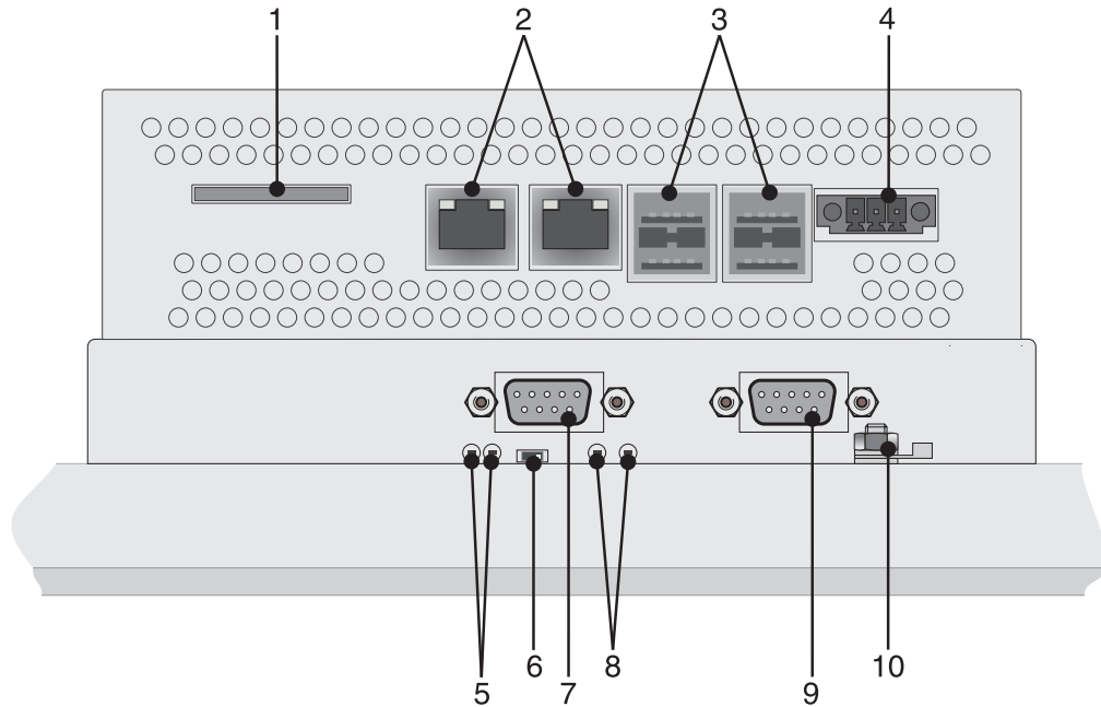
Figure 4-3 Rear view RS-422 / RS-485, RS-232
