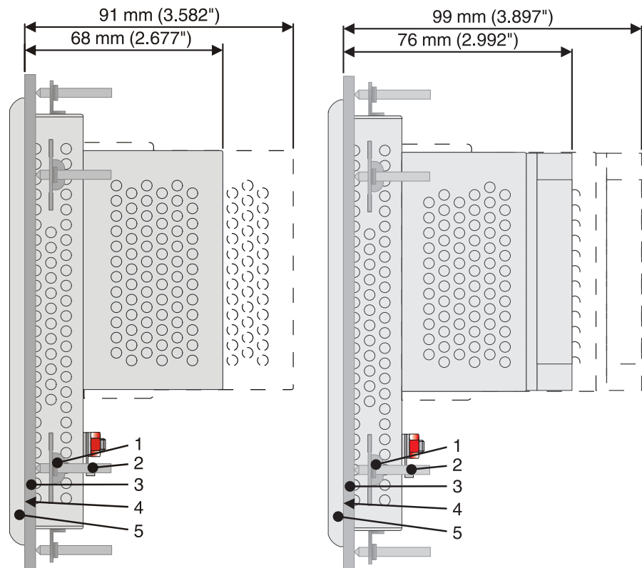
Figure 2-19 TP070ZTW / TP070GTW
