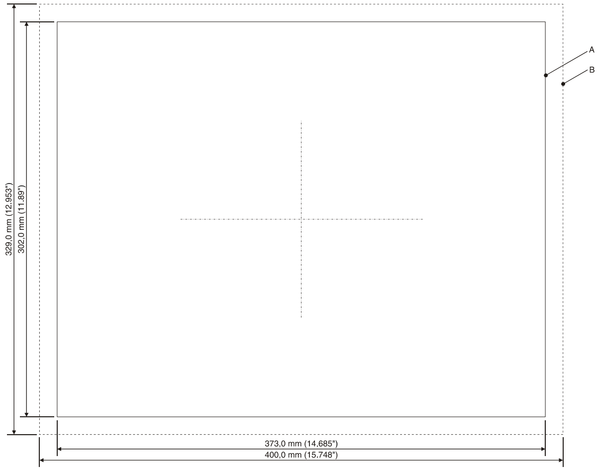
Figure 2-16 TP150ZTX / TP150GTX
