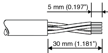
Figure 2-26 Preparing the cable
