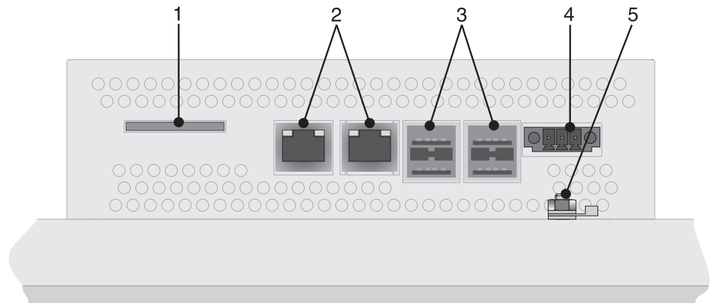
Figure 4-1 Rear view
