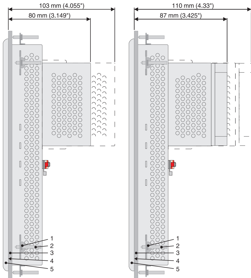
Figure 2-21 TP105ZTS / TP105GTS
