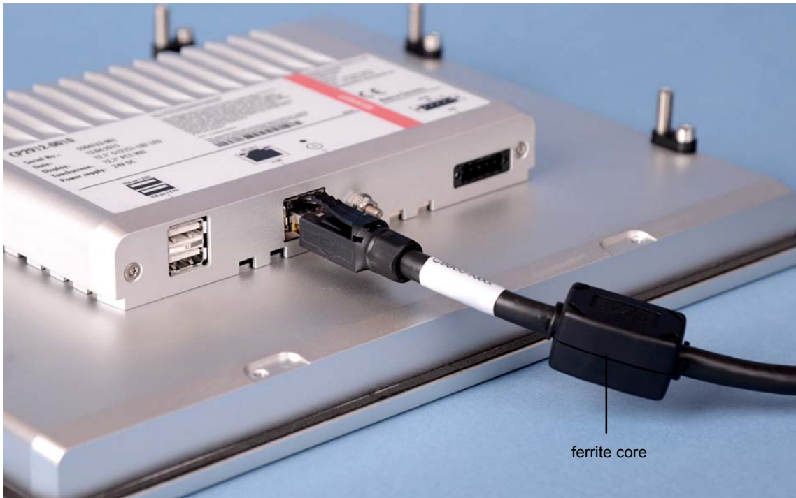
CP-Link 4 cable connection
