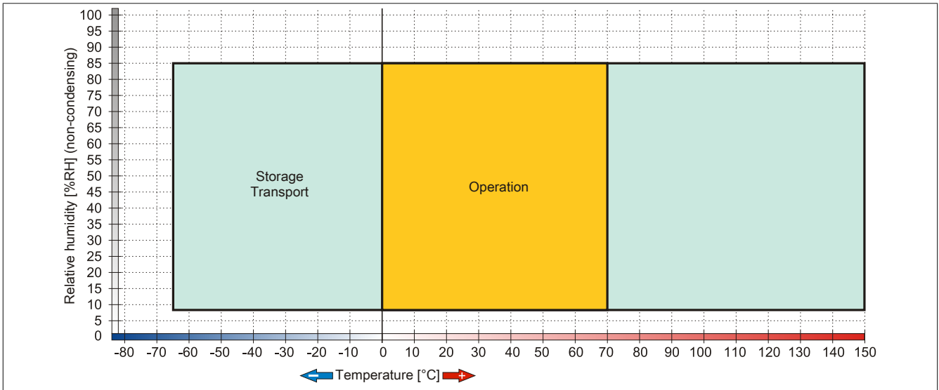
Figure 145: 5CFCRD.xxxx-04 - Temperature/Humidity diagram for CompactFlash cards
