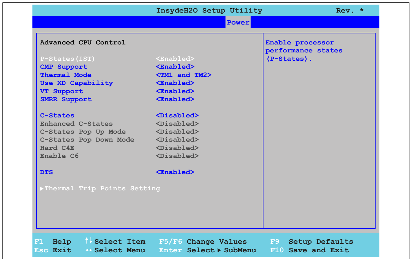
Figure 122: US15W Power - Advanced - CPU Control
