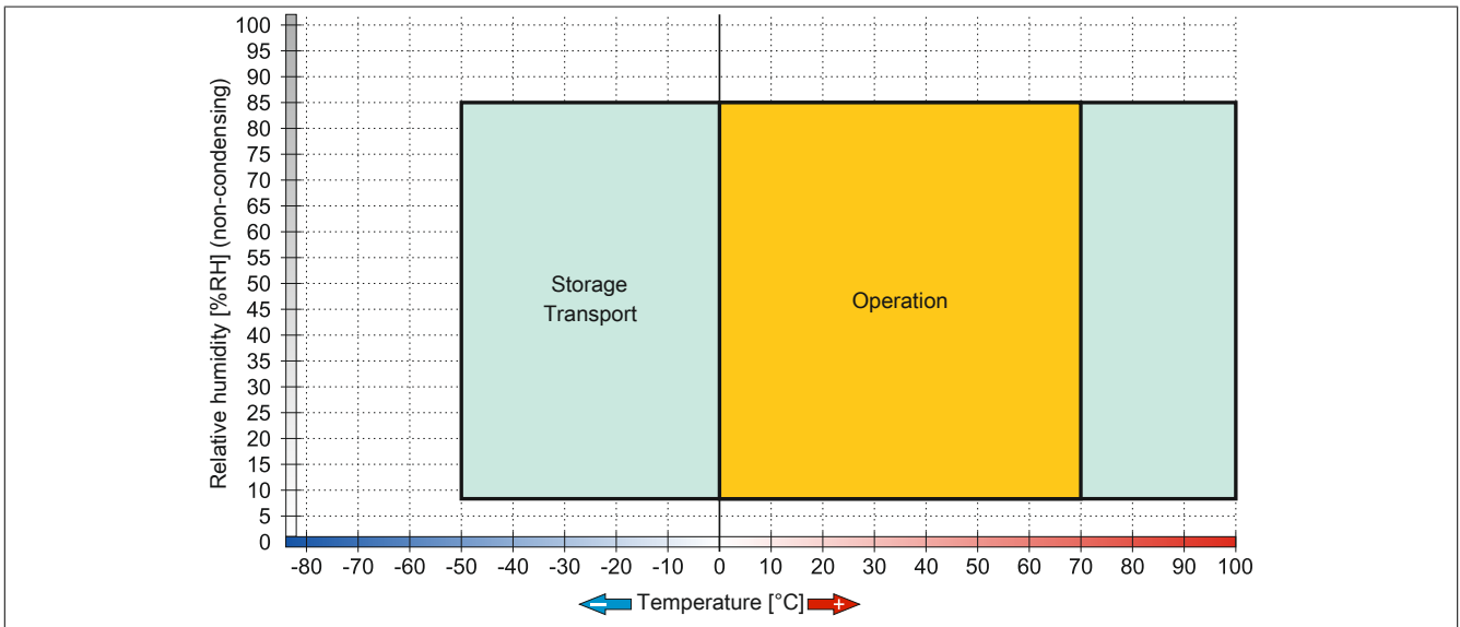
Figure 141: 5CFCRD.xxxx-06 - Temperature/Humidity diagram for CompactFlash cards
