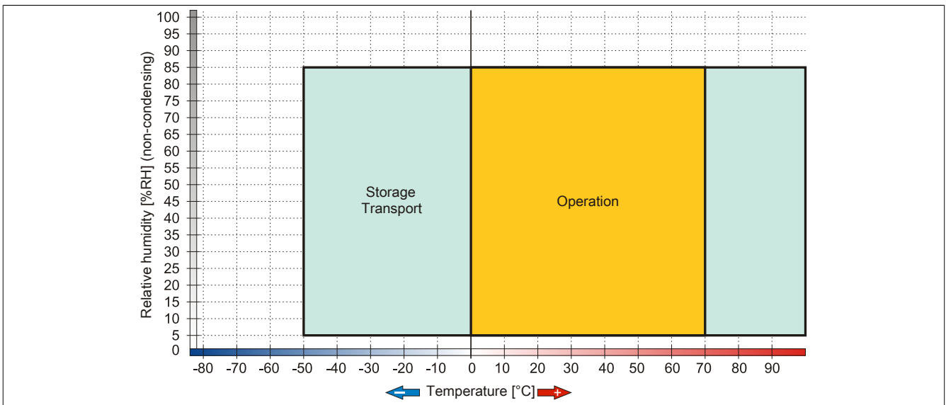
Figure 158: 5MMUSB.xxx-01 - Temperature/Humidity diagram
