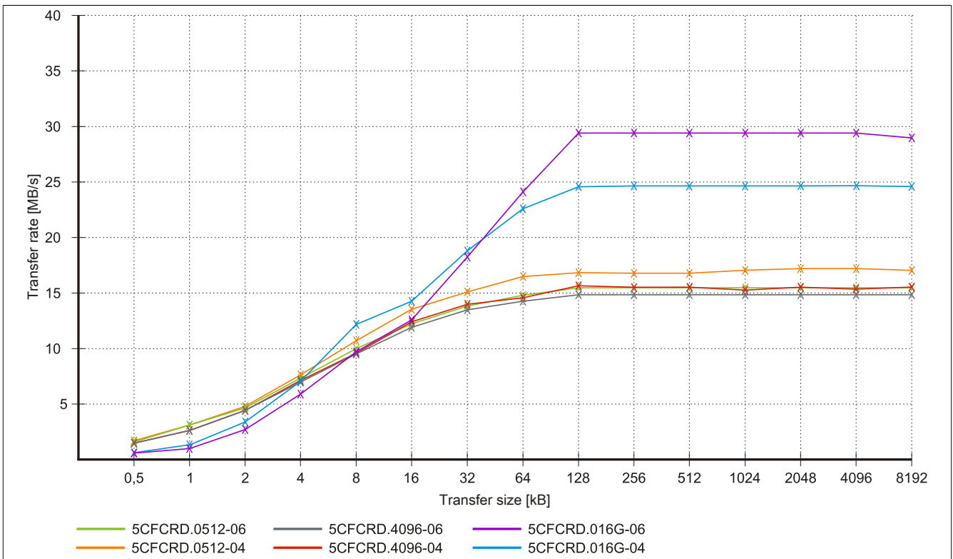
Figure 144: ATTO Disk Benchmark v2.34 write comparison - 5CFCRD.xxxx-04 and 5CFCRD.xxxx-06
