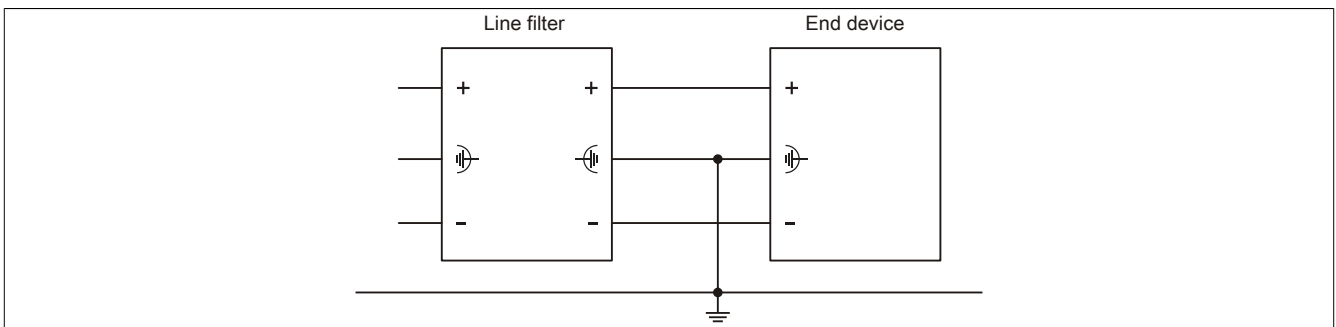
Figure 161: Connection example
