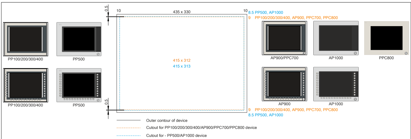
Figure 176: Mounting compatibility - 15" device - Horizontal1
