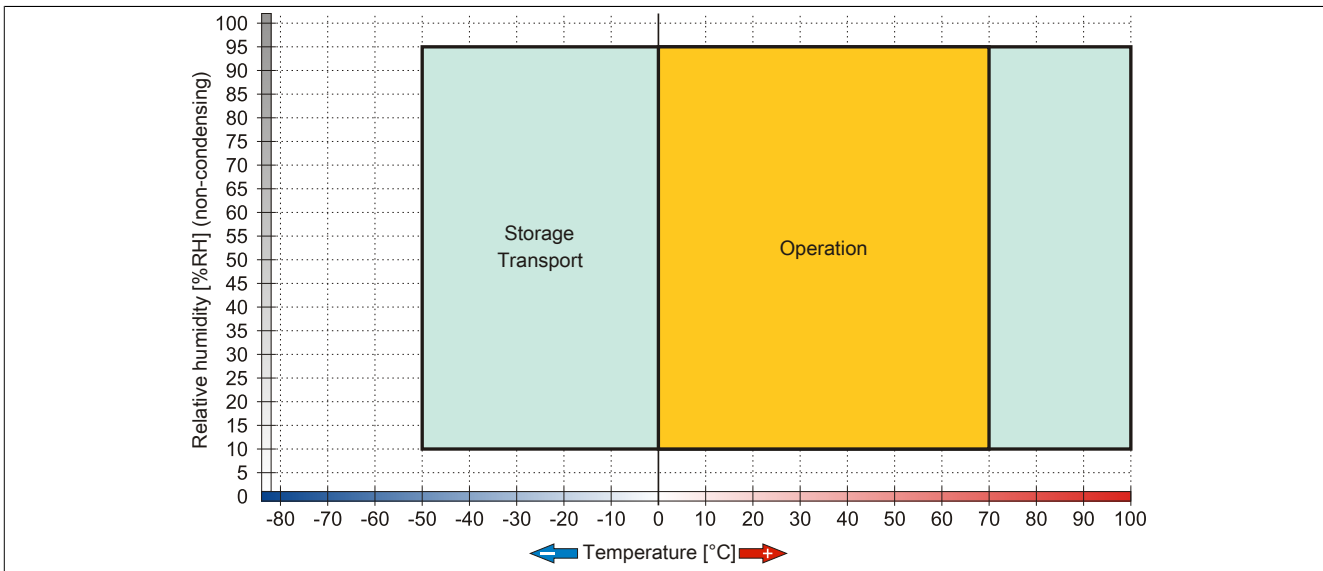
Figure 149: 5CFCRD.xxxx-03 - Temperature/Humidity diagram for CompactFlash cards
