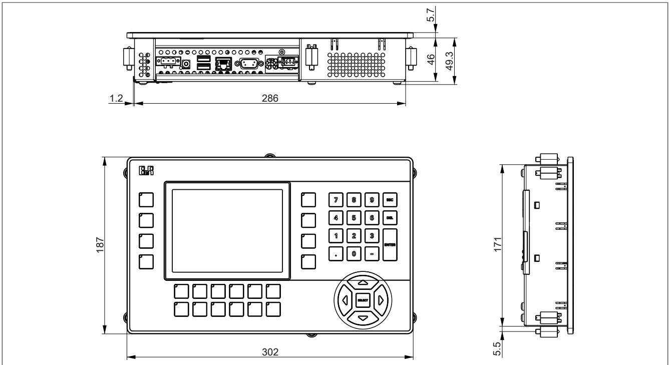
Figure 20: 5PP552.0573-00 - Dimensions
