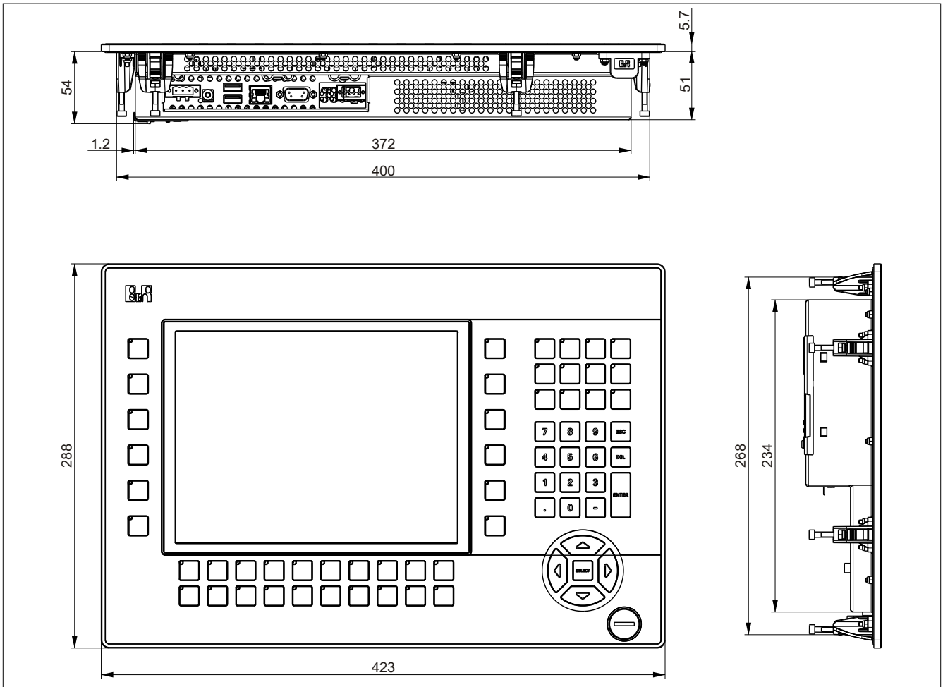
Figure 35: 5PP582.1043-00 - Dimensions
