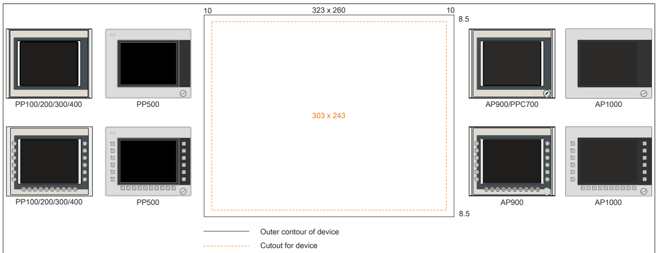
Figure 172: Mounting compatibility - 10.4" device - Horizontal1
