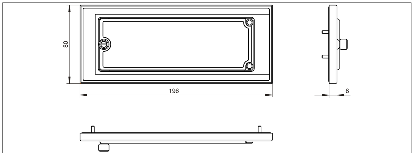
Figure 155: 5A5003.03 - Dimensions
