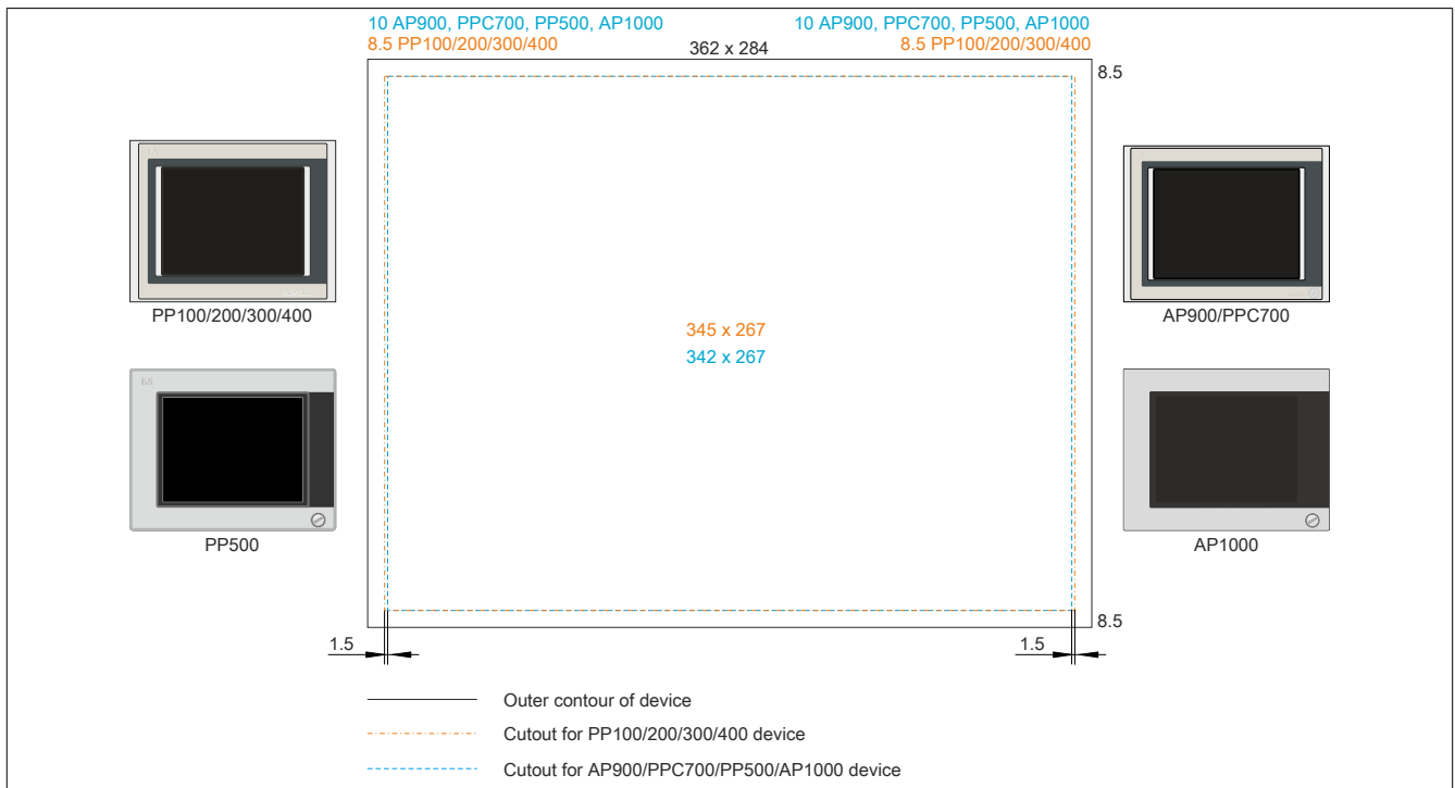
Figure 175: Mounting compatibility - 12.1" device - Horizontal1
