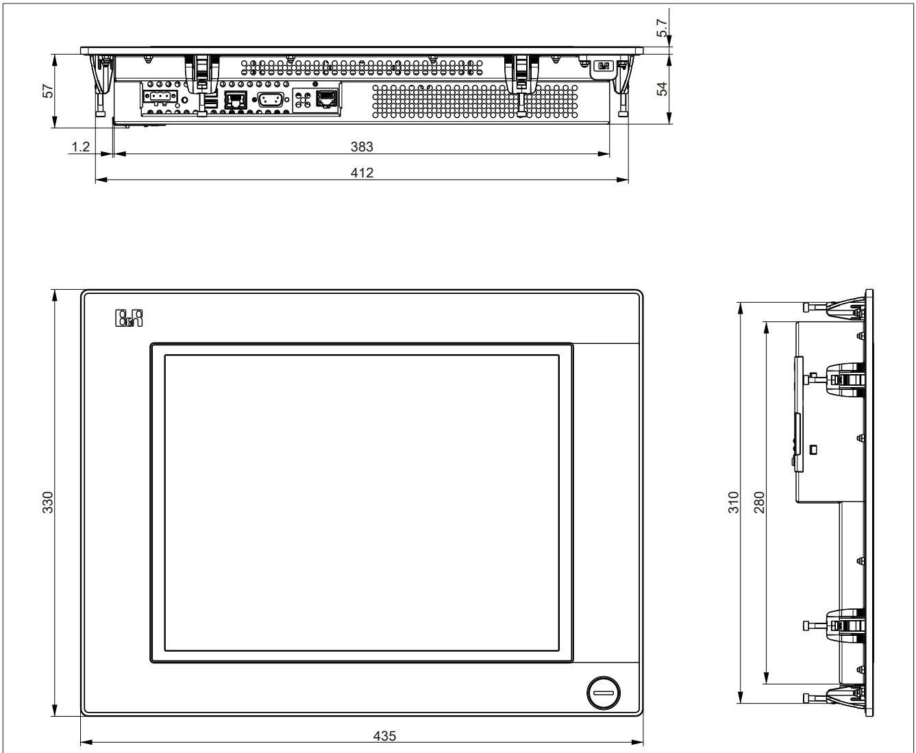
Figure 41: 5PP520.1505-00 - Dimensions
