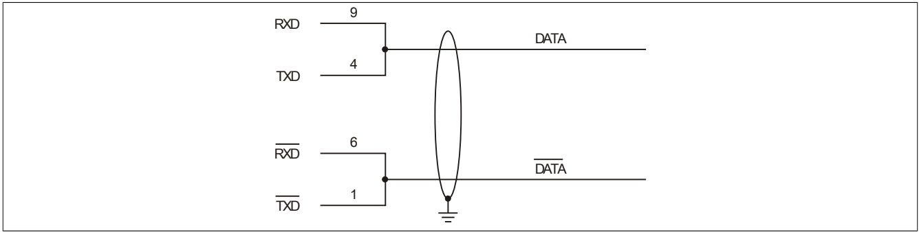
Figure 52: RS232/RS422/RS485 interface - Operation in RS485 mode
