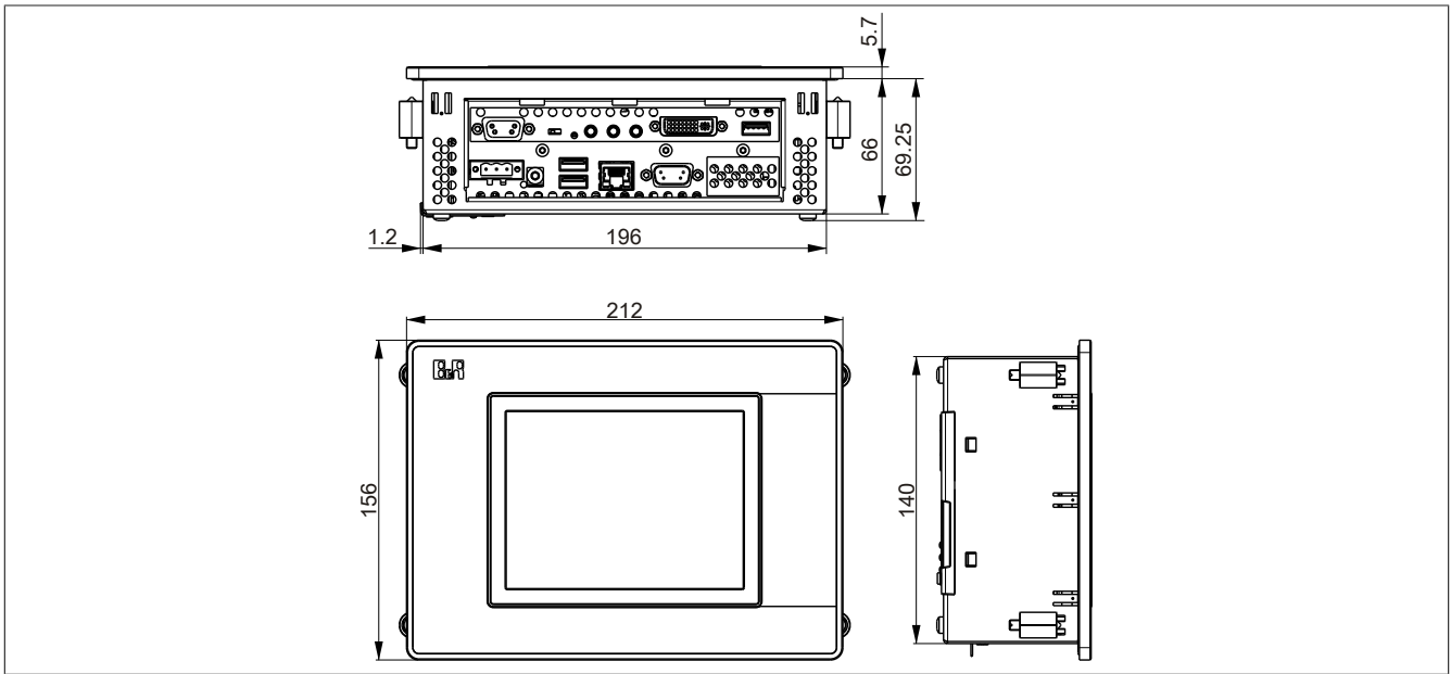
Figure 14: 5PP520.0573-01 - Dimensions
