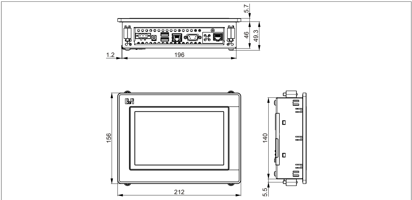
Figure 23: 5PP520.0702-00 - Dimensions
