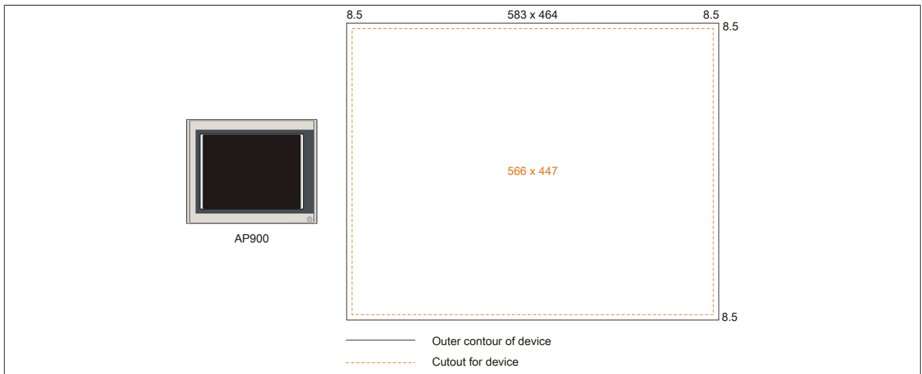
Figure 180: Mounting compatibility - 21.3" device - Horizontal1
