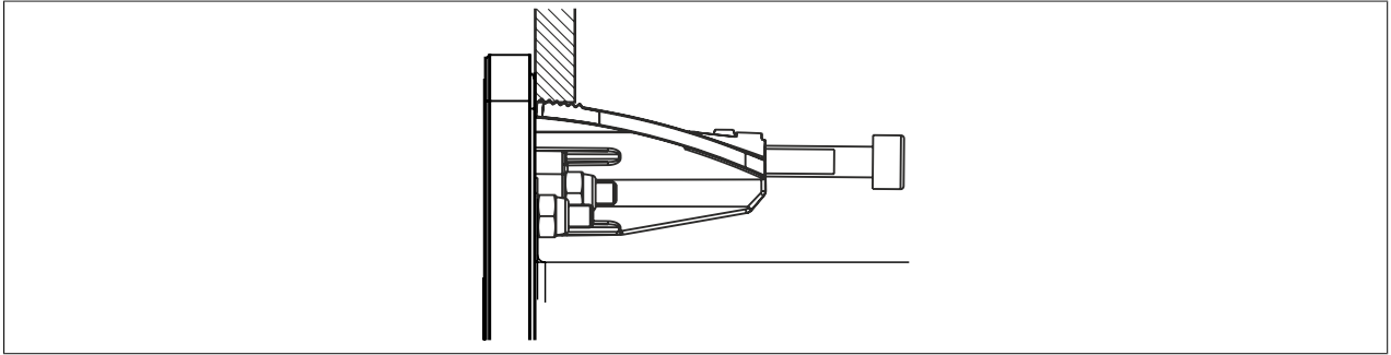
Figure 55: Device with clamping block inserted in cutout
