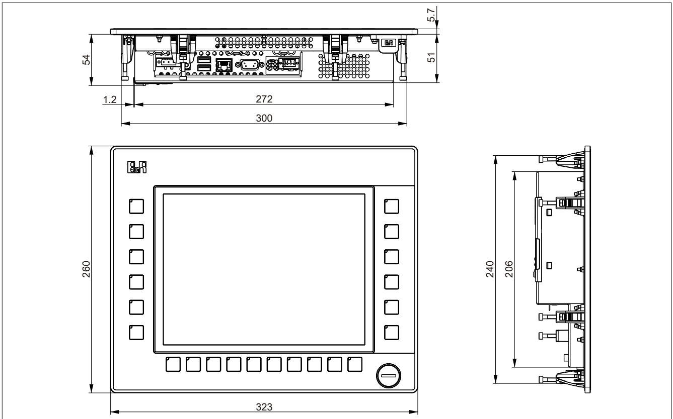
Figure 29: 5PP580.1043-00 - Dimensions
