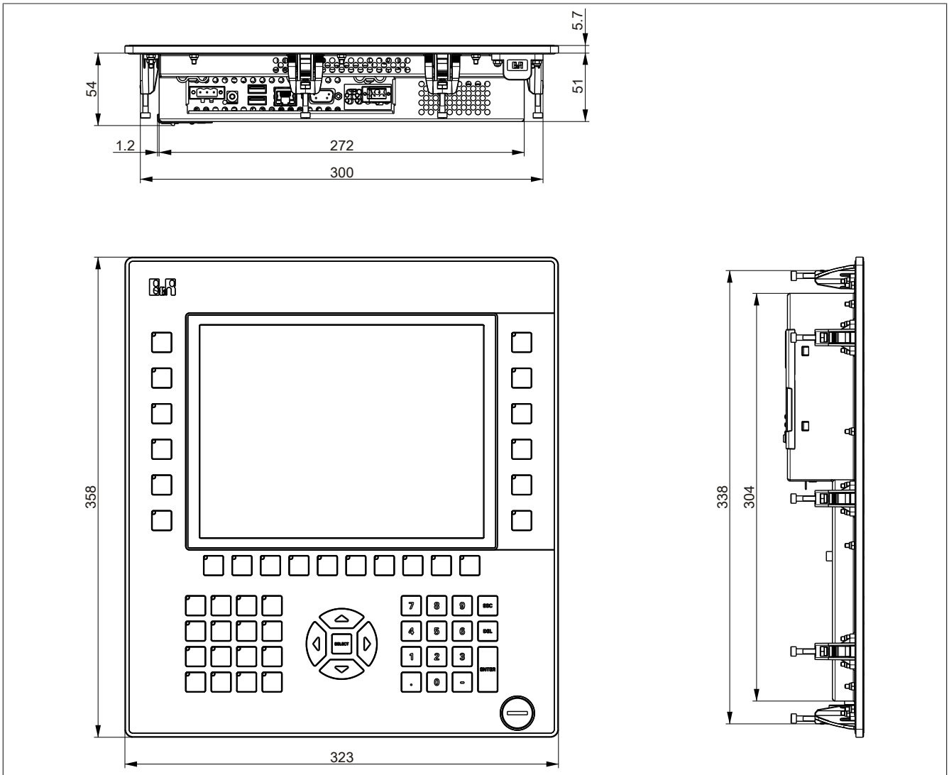
Figure 32: 5PP581.1043-00 - Dimensions
