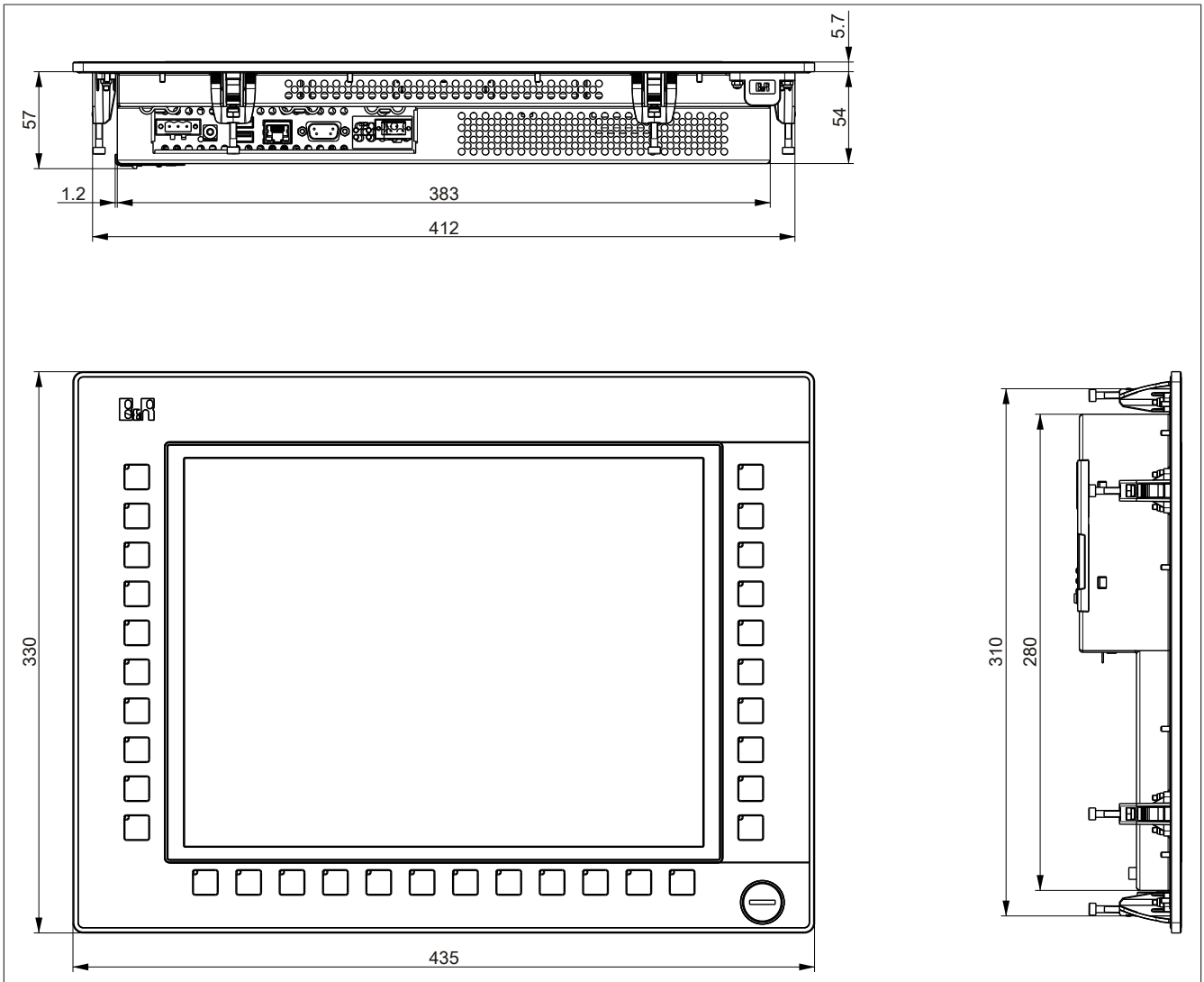
Figure 44: 5PP580.1505-00 - Dimensions
