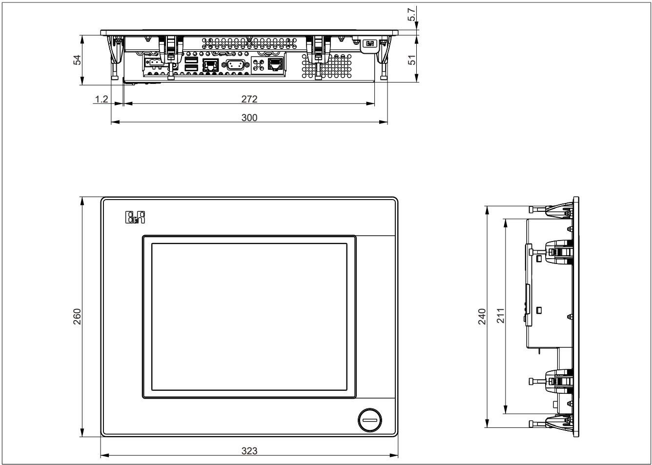
Figure 26: 5PP520.1043-00 - Dimensions
