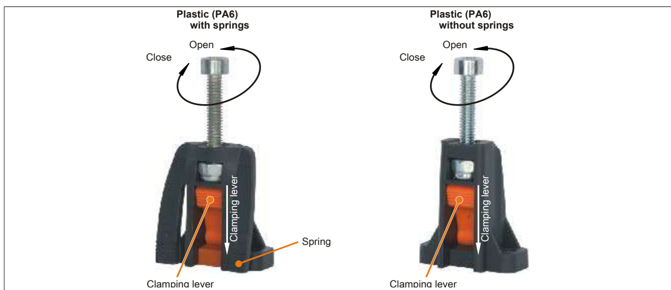
Figure 54: Clamping blocks
