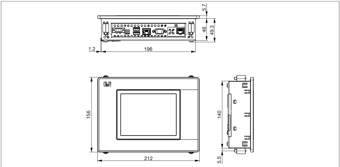
Figure 11: 5PP520.0573-00 - Dimensions
