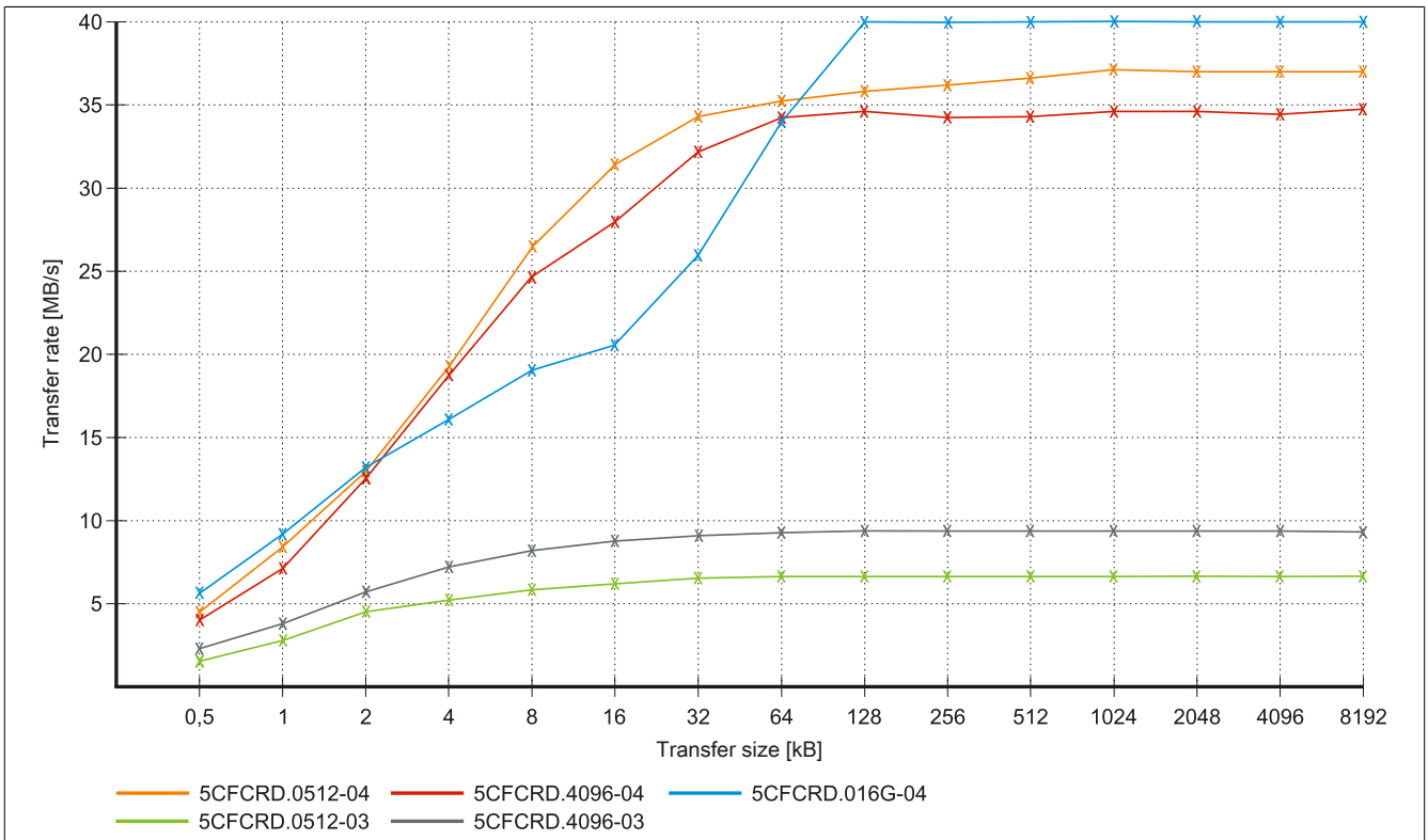
Figure 147: ATTO Disk Benchmark v2.34 read comparison - 5CFCRD.xxxx-03 and 5CFCRD.xxxx-04
