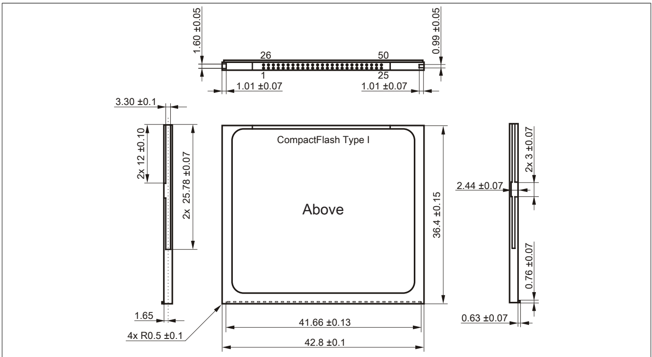
Figure 142: Type I CompactFlash card - Dimensions
