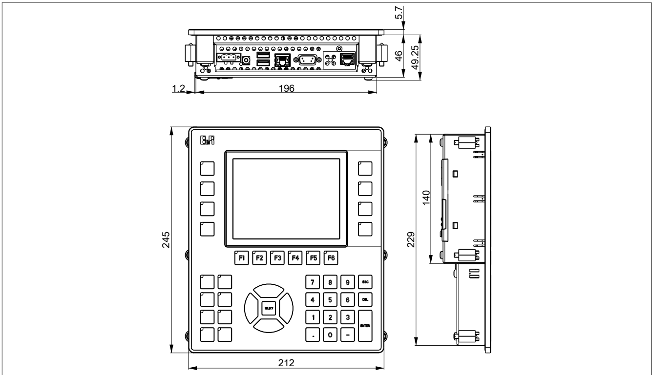
Figure 17: 5PP551.0573-00 - Dimensions
