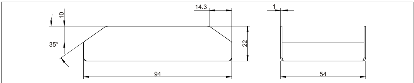
Figure 159: 5AC804.MFLT-00 - Dimensions
