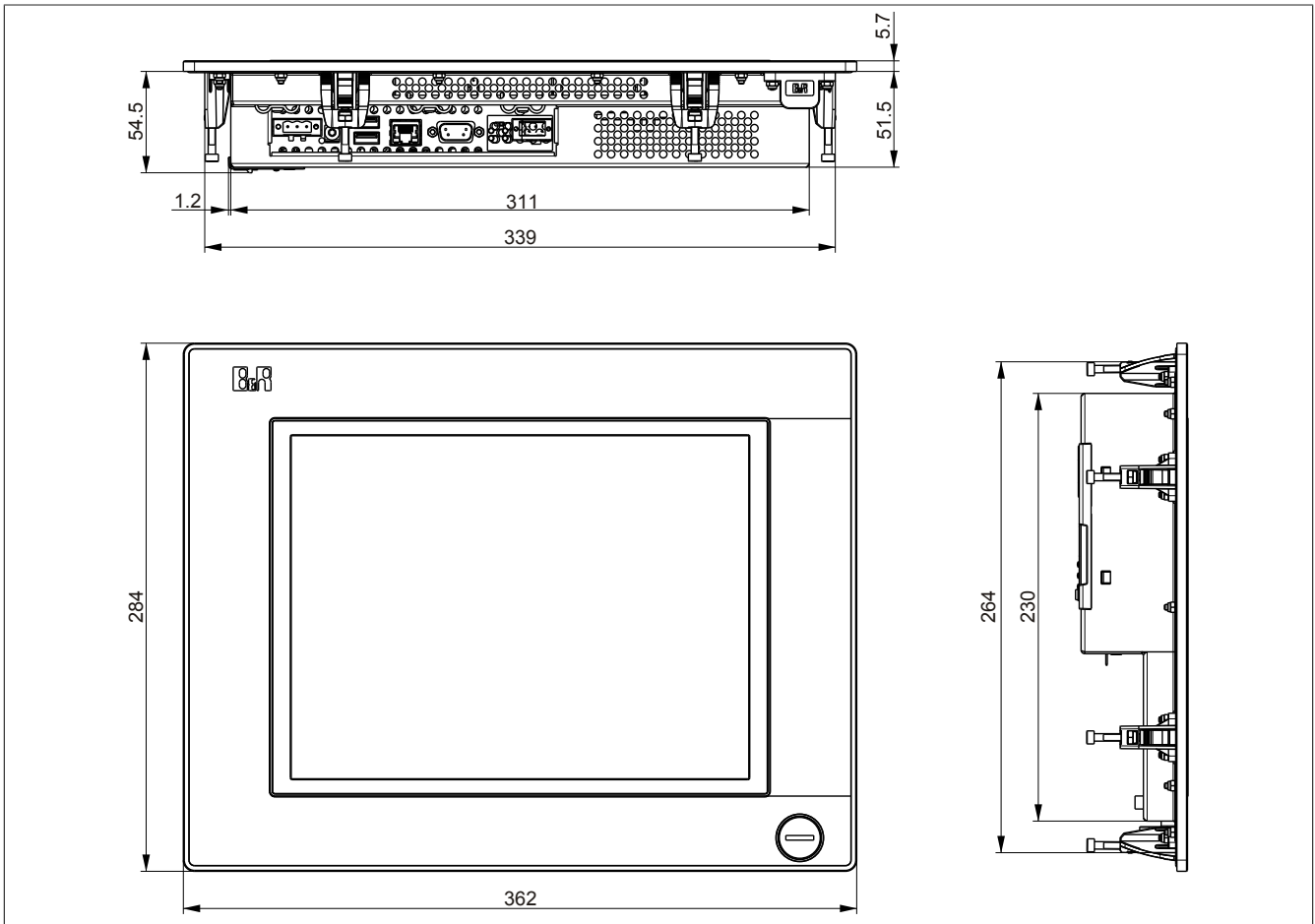
Figure 38: 5PP520.1214-00 - Dimensions
