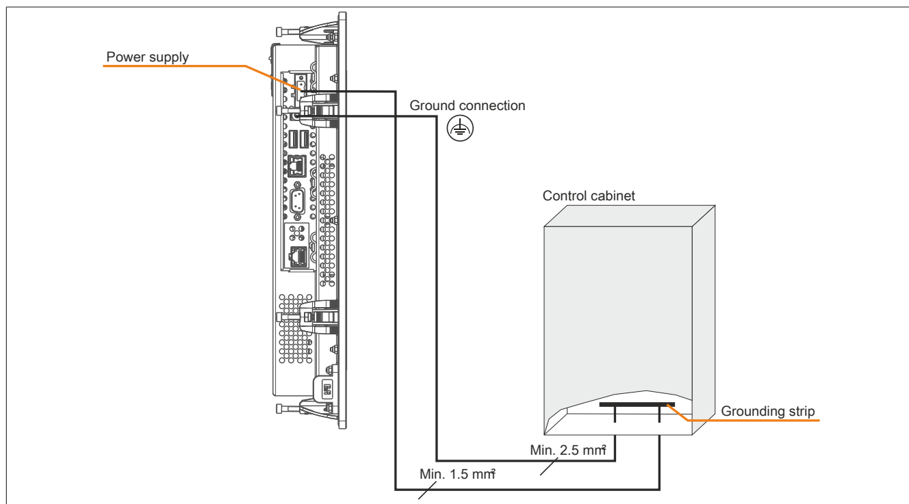
Figure 71: Grounding concept
