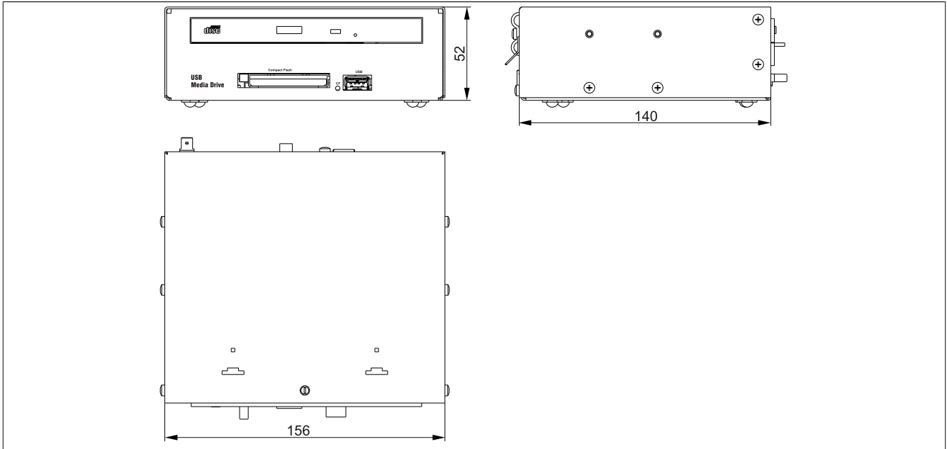
Figure 151: 5MD900.USB2-02 - Dimensions
